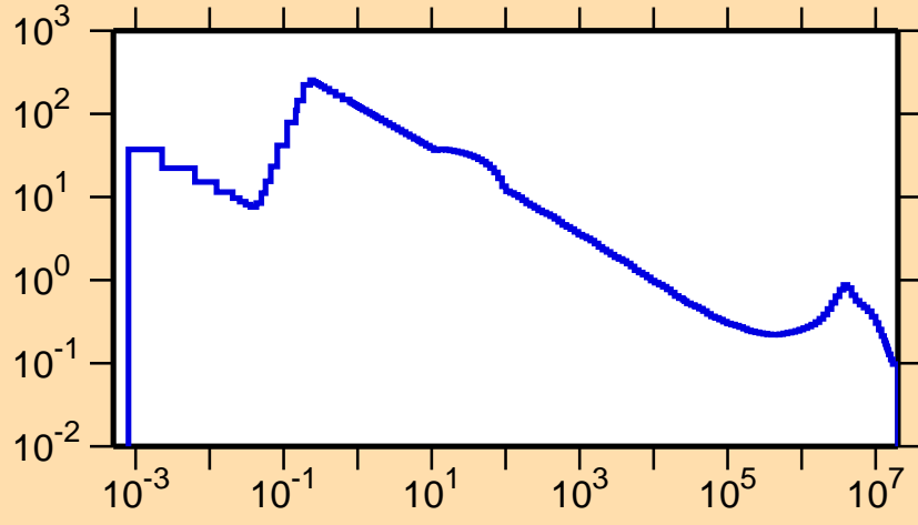
\sigma vs. E for ^{137}\text{Pm}(n,p)
