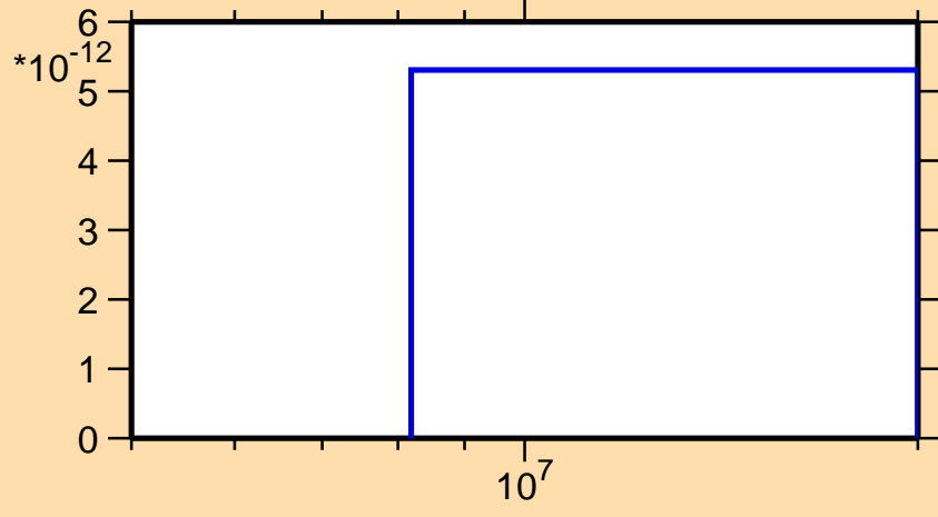
\sigma vs. E for ^{137}\text{Pm}(n,pt)
