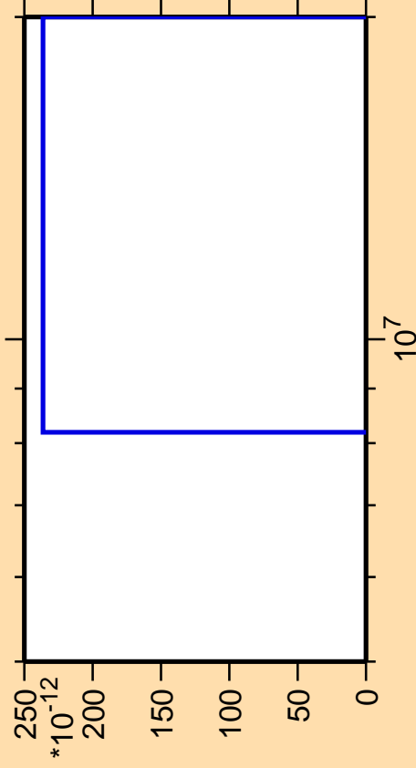
\Delta\sigma/\sigma vs. E for ^{137}\text{Pm} (mt 11)
