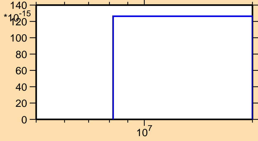
\sigma vs. E for ^{137}\text{Pm} (mt 34)
