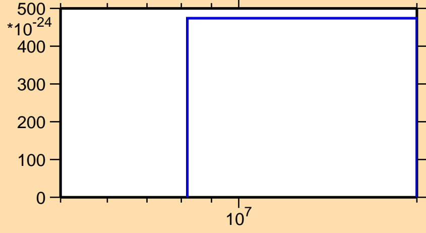
\sigma vs. E for ^{137}\text{Pm} (mt 11)
