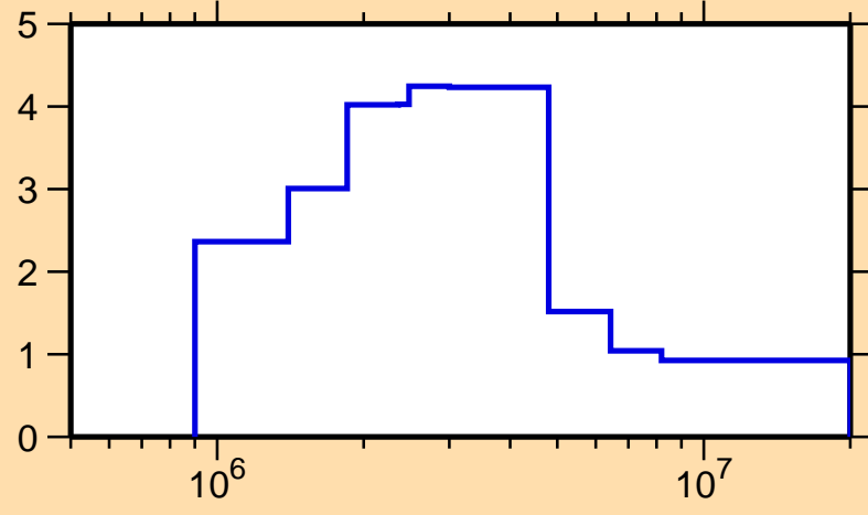
\Delta\sigma/\sigma vs. E for ^{137}\text{Pm}(n,\text{el.})
