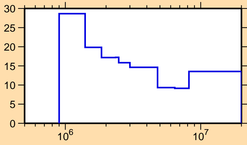
\Delta\sigma/\sigma vs. E for ^{137}\text{Pm}(n,n\text{cont.})
