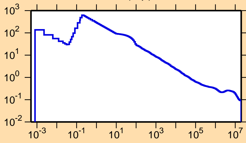
\sigma vs. E for ^{138}\text{Pm}(n,p)
