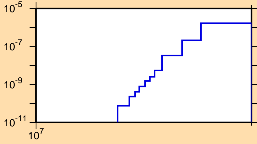
\sigma vs. E for ^{138}\text{Pm} (mt 45)
