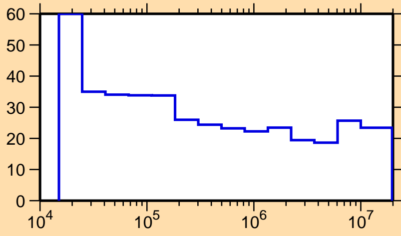
\Delta\sigma/\sigma vs. E for ^{138}\text{Pm}(n,n_1)
