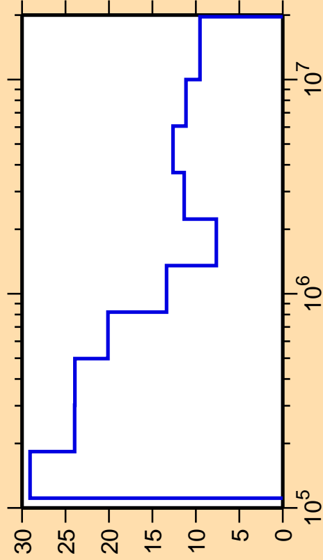
\Delta\sigma/\sigma vs. E for ^{138}\text{Pm}(n,n_2)
