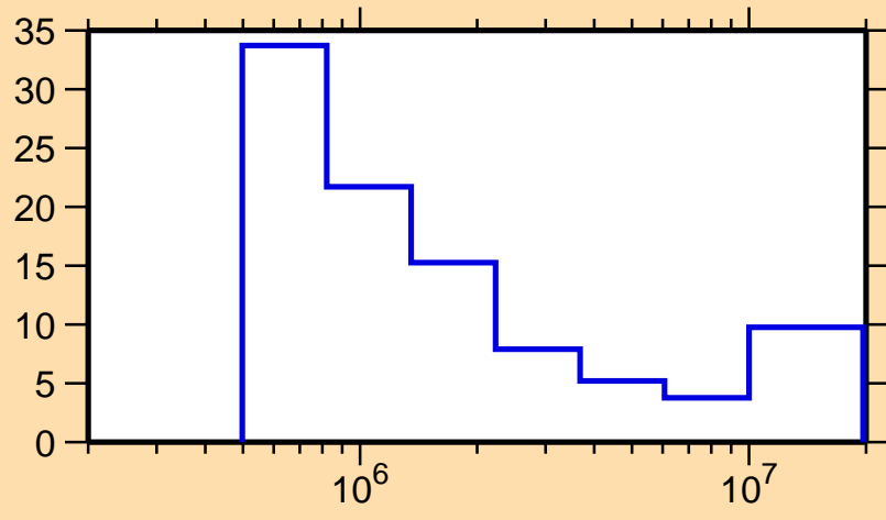
\Delta\sigma/\sigma vs. E for ^{138}\text{Pm}(n,ncont.)
