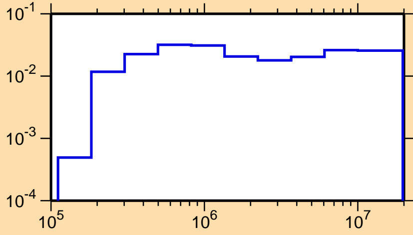
\sigma vs. E for ^{138}\text{Pm}(n,n_2)
