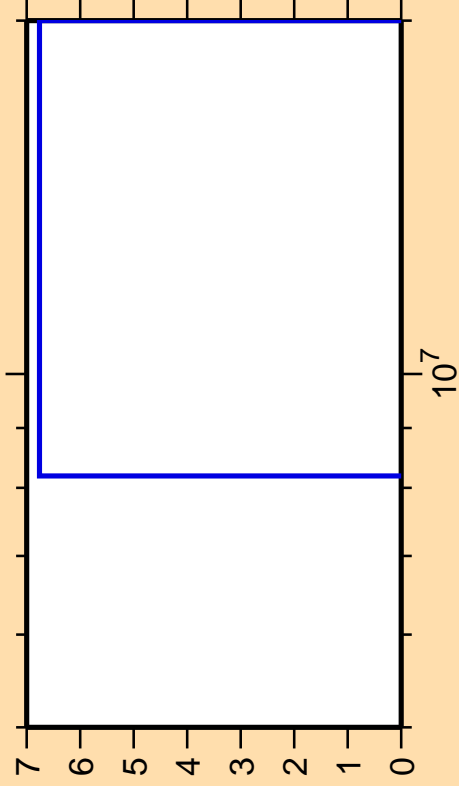
\Delta\sigma/\sigma vs. E for ^{138}\text{Pm}(n,n\text{cont.})
