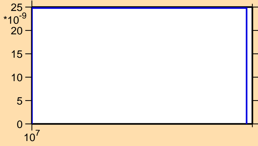
\sigma vs. E for ^{138}\text{Pm}(n,\text{pd})
