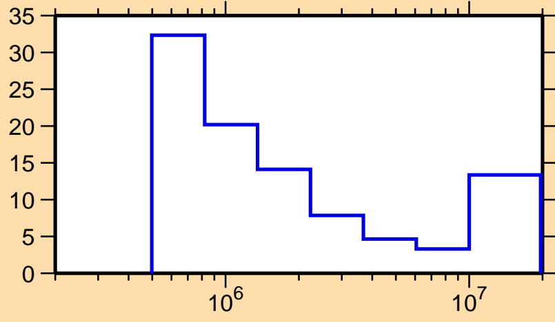
\Delta\sigma/\sigma vs. E for ^{138}\text{Pm}(n,ncont.)
