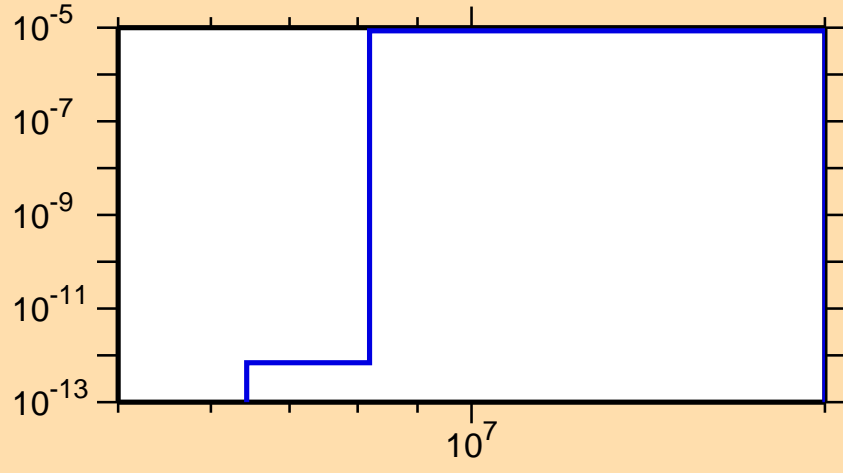
\sigma vs. E for ^{138}\text{Pm}(n,\text{He}3)
