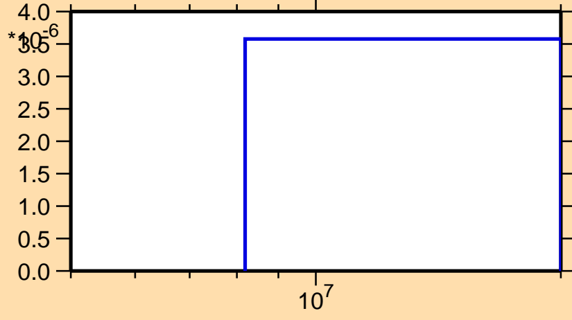
\sigma vs. E for ^{138}\text{Pm}(n,nd)
