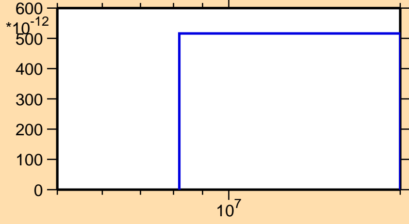
\sigma vs. E for ^{138}\text{Pm}(n,\text{pt})
