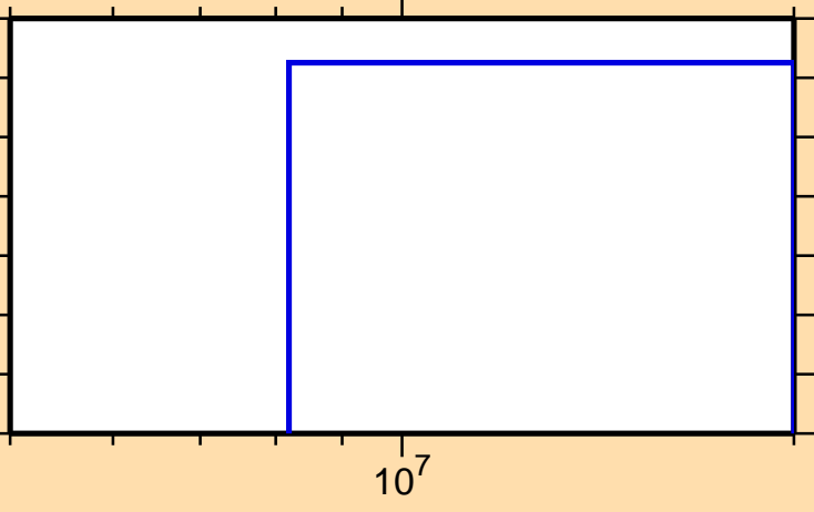
\sigma vs. E for ^{138}\text{Pm} (mt 45)
