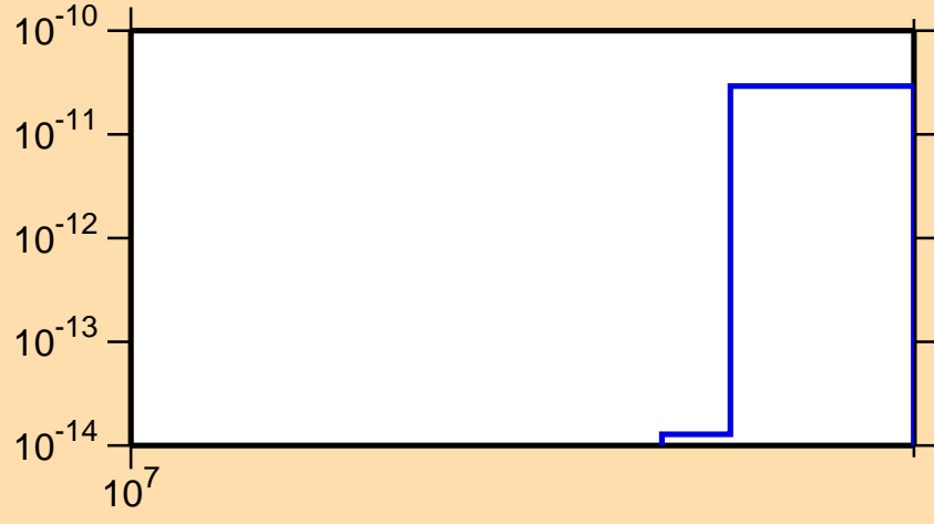
\sigma vs. E for ^{139}\text{Pm}(n,pt)
