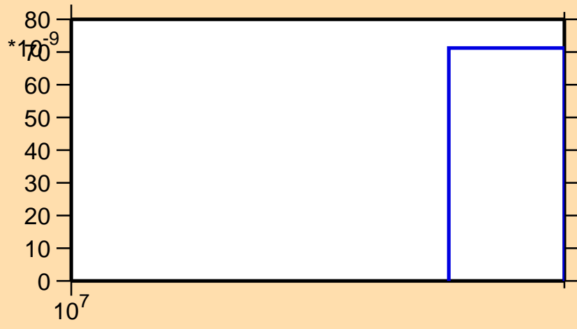
\sigma vs. E for ^{139}\text{Pm}(n,3n)
