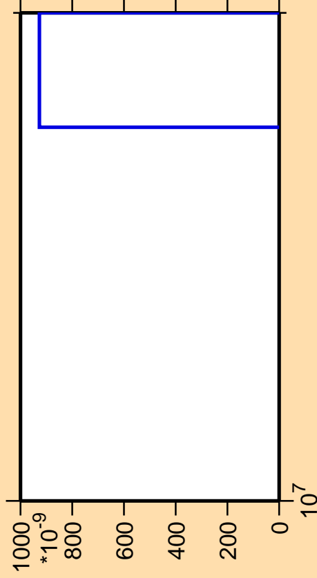
\Delta\sigma/\sigma vs. E for ^{139}\text{Pm} (mt 11)
