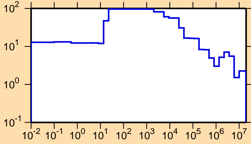
\Delta\sigma/\sigma vs. E for ^{139}\text{Pm}(n,el.)
