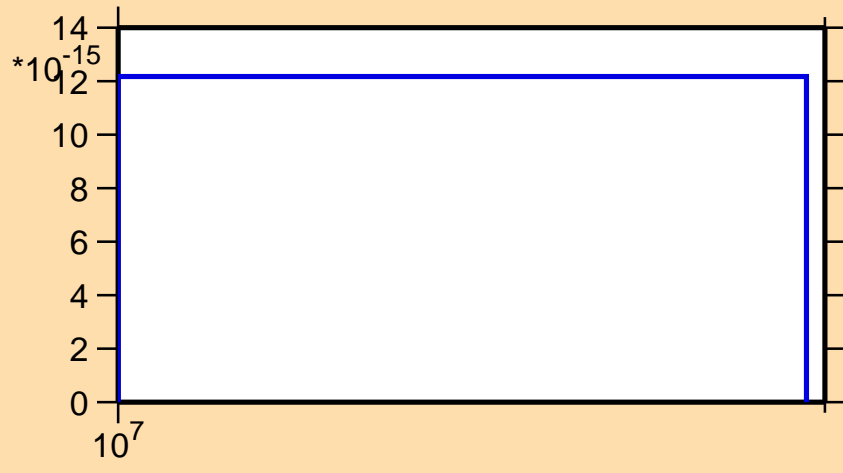
\sigma vs. E for ^{139}\text{Pm} (mt 34)
