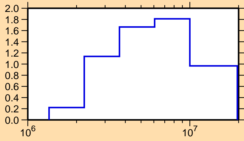
\sigma vs. E for ^{139}\text{Pm}(n,n\text{cont.})
