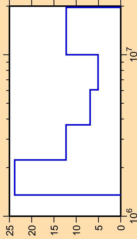
\Delta\sigma/\sigma vs. E for ^{139}\text{Pm}(n,n\text{cont.})
