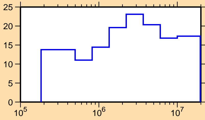
\Delta\sigma/\sigma vs. E for ^{139}\text{Pm}(n,n_1)
