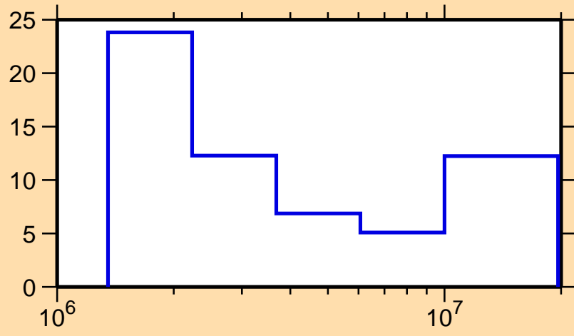
\Delta\sigma/\sigma vs. E for ^{139}\text{Pm}(n,ncont.)
