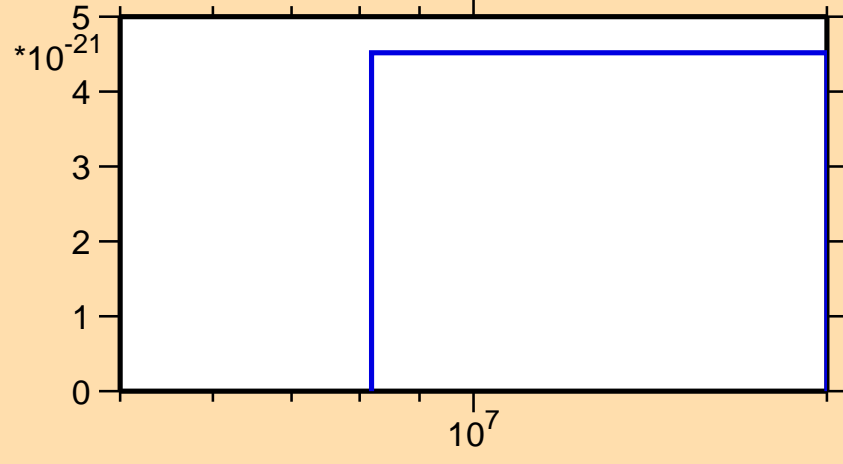
\sigma vs. E for ^{139}\text{Pm} (mt 11)
