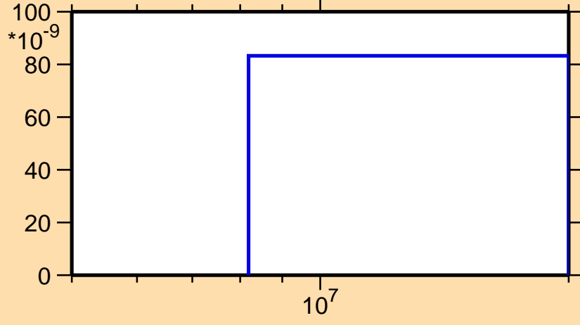
\sigma vs. E for ^{139}\text{Pm}(n,nd)
