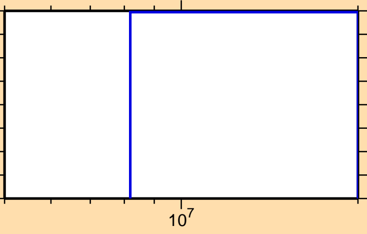
\sigma vs. E for ^{139}\text{Pm}(n,2np)
