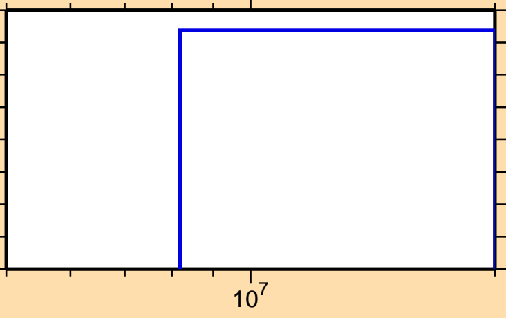
\sigma vs. E for ^{139}\text{Pm}(n,\text{pd})
