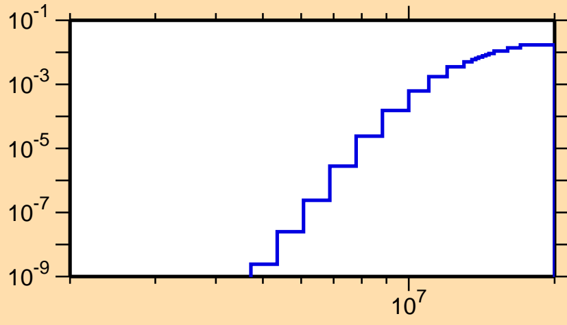
\sigma vs. E for ^{140}\text{Pm}(n,d)
