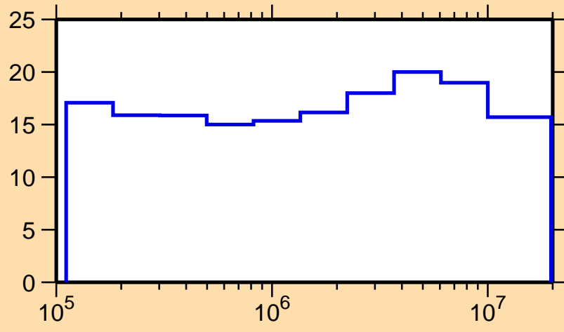
\Delta\sigma/\sigma vs. E for ^{140}\text{Pm}(n,n_1)
