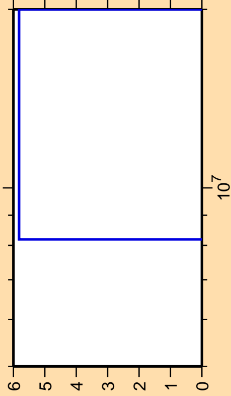
\Delta\sigma/\sigma vs. E for ^{140}\text{Pm}(n,2n)
