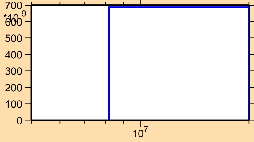
\sigma vs. E for ^{140}\text{Pm}(n,nd)
