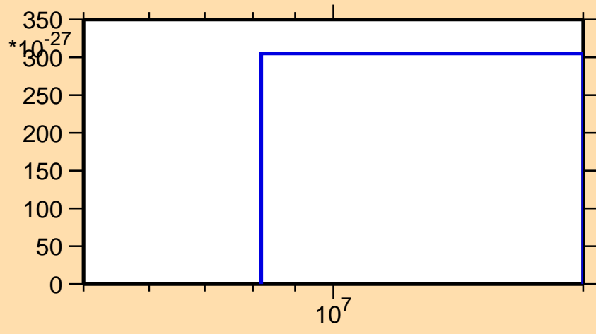
\sigma vs. E for ^{140}\text{Pm}(\text{mt } 11)
