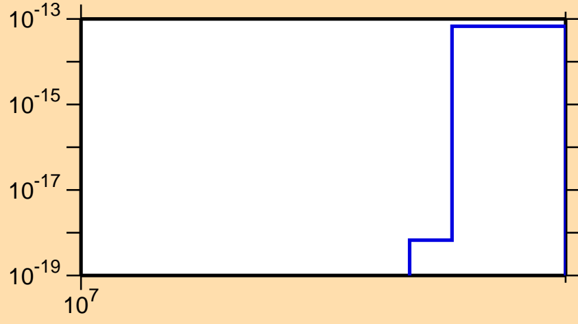
\sigma vs. E for ^{141}\text{Pm}(n,\text{pt})
