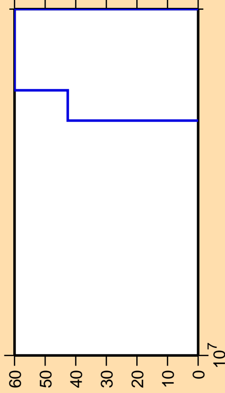
\Delta\sigma/\sigma vs. E for ^{141}\text{Pm} (mt117)
