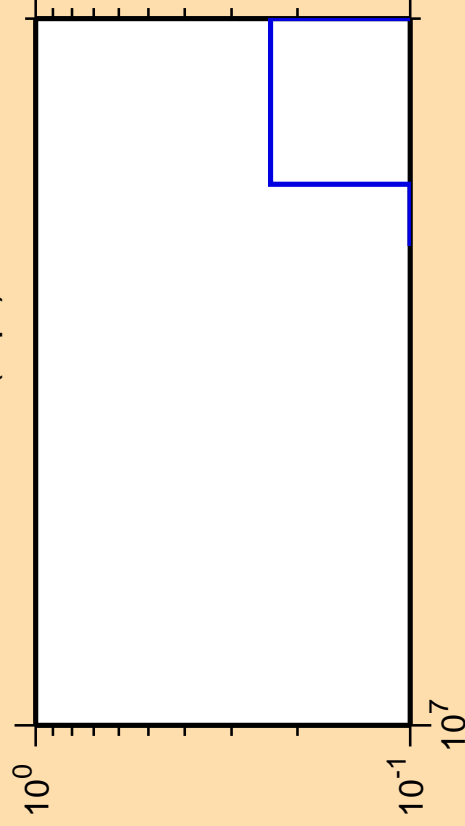
\Delta\sigma/\sigma vs. E for ^{141}\text{Pm}(n,\text{pt})
