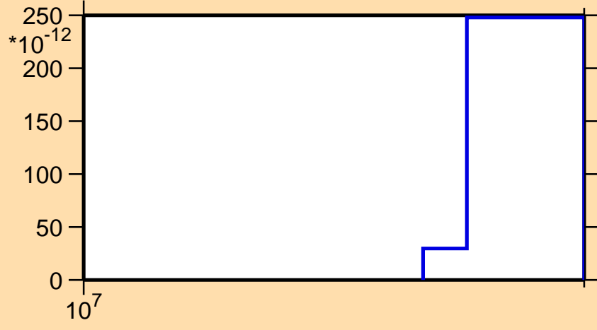
\sigma vs. E for ^{141}\text{Pm} (mt117)
