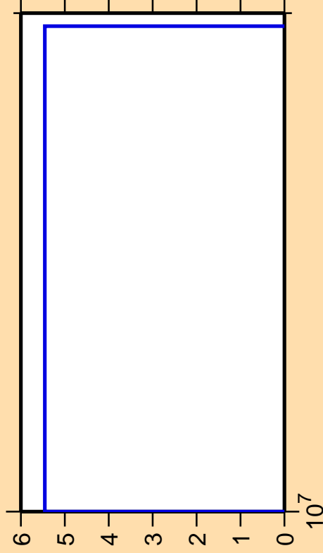
\Delta\sigma/\sigma vs. E for ^{141}\text{Pm}(\text{mt117})
