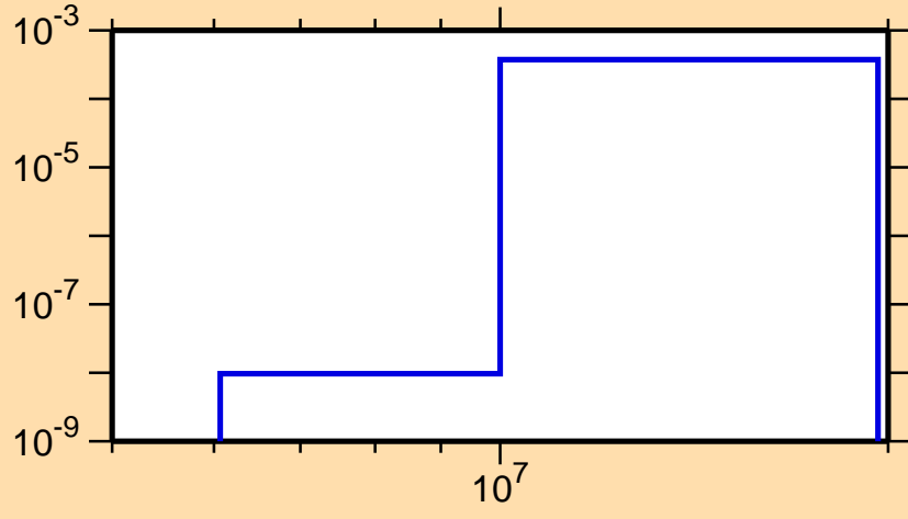
\sigma vs. E for ^{142}\text{Pm}(n,n\alpha)
