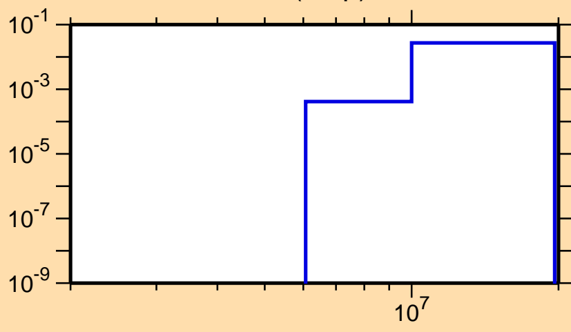
\sigma vs. E for ^{142}\text{Pm}(n,np)
