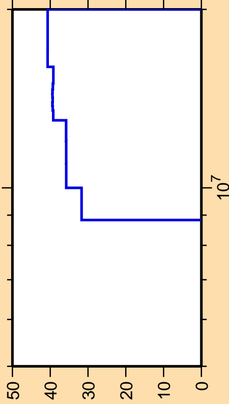
\Delta\sigma/\sigma vs. E for ^{143}\text{Pm}(n,\gamma)
