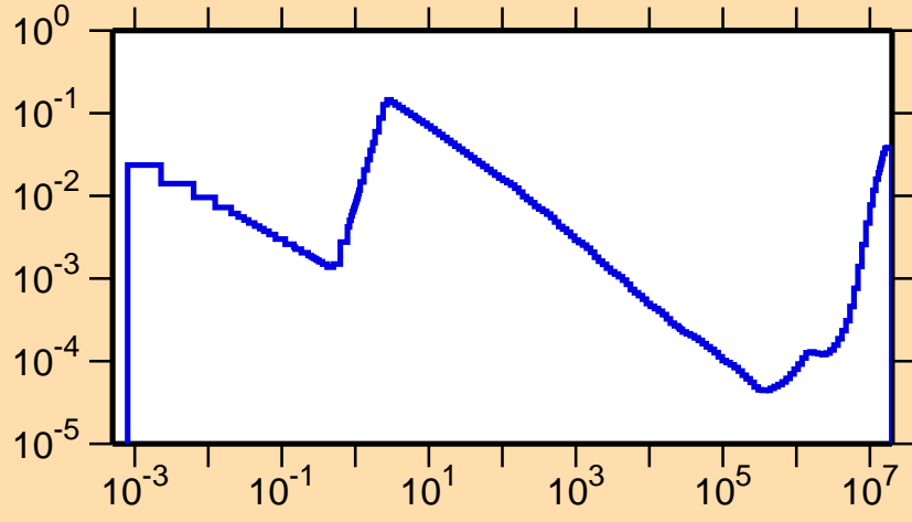
\sigma vs. E for ^{144}\text{Pm}(n,\alpha)
