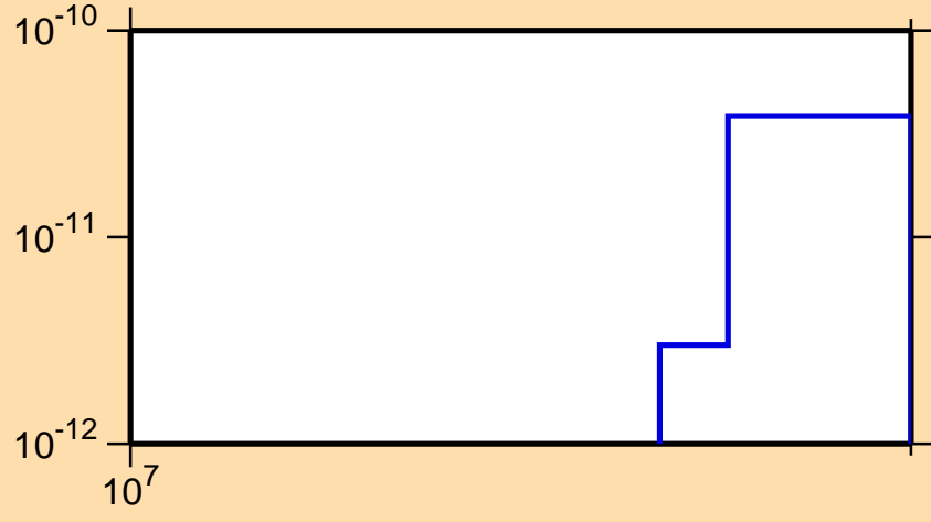
\sigma vs. E for ^{144}\text{Pm} (mt 45)
