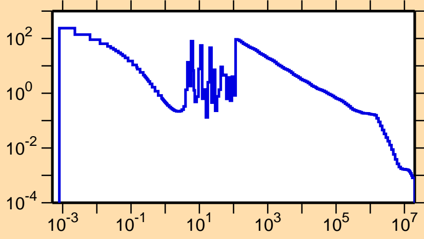
\sigma vs. E for ^{144}\text{Pm}(n,\gamma)
