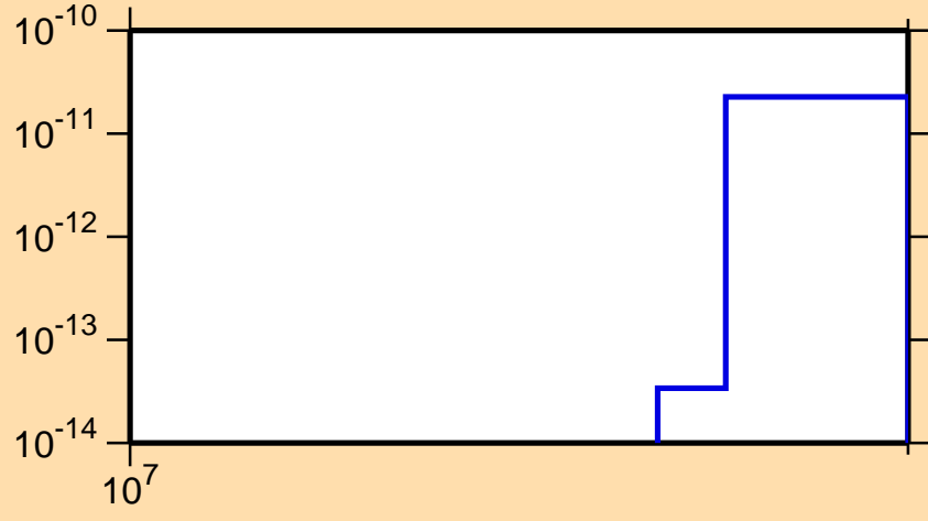
\sigma vs. E for ^{144}\text{Pm} (mt 34)
