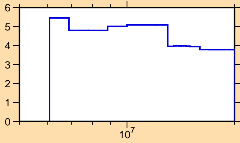
\Delta\sigma/\sigma vs. E for ^{144}\text{Pm}(n,\text{nonel.})
