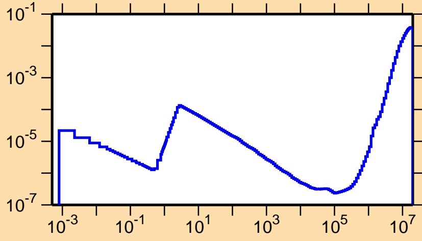
\sigma vs. E for ^{144}\text{Pm}(n,p)
