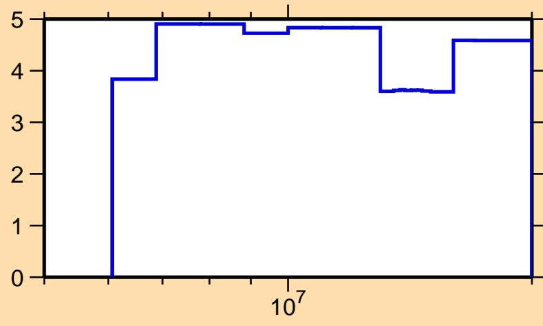
\Delta\sigma/\sigma vs. E for ^{144}\text{Pm}(n,\text{el.})
