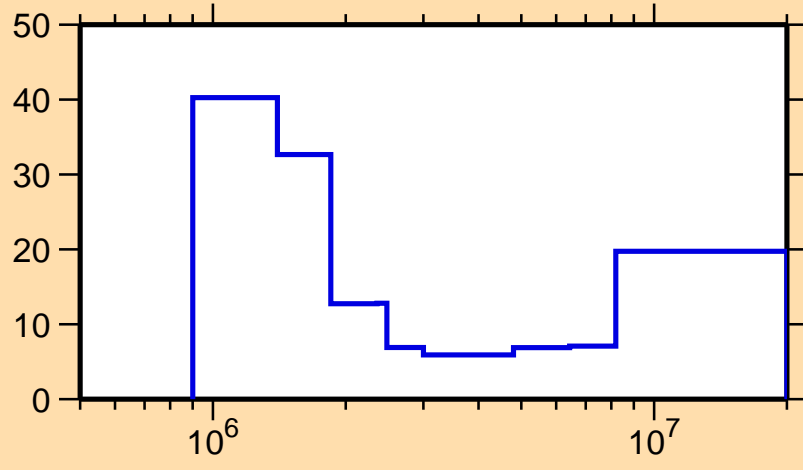
\Delta\sigma/\sigma vs. E for ^{144}\text{Pm}(n,ncont.)
