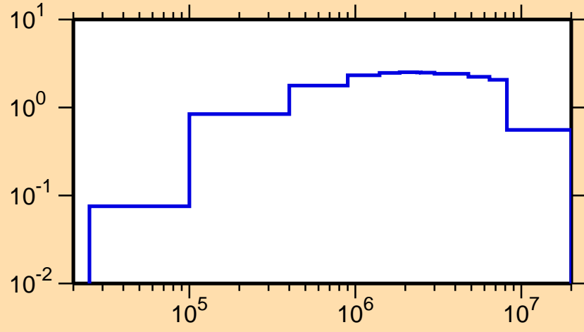
\sigma vs. E for ^{144}\text{Pm}(n,\text{inel.})
