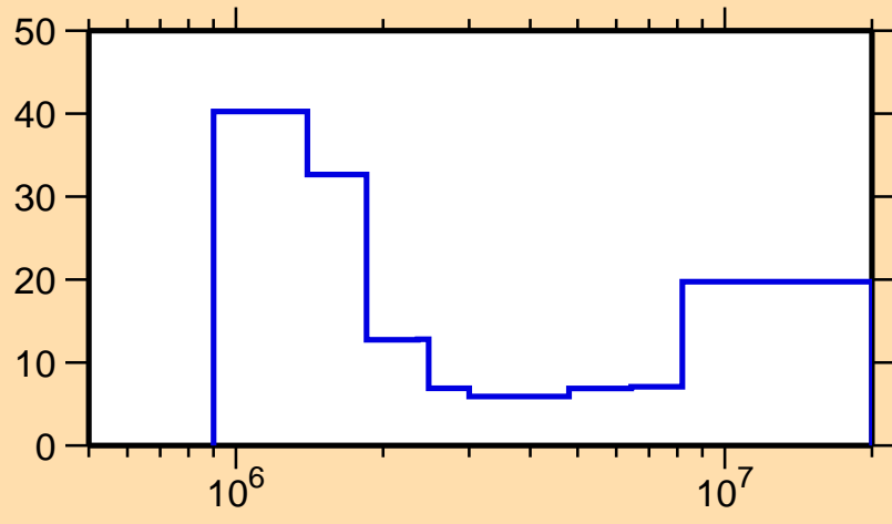
\Delta\sigma/\sigma vs. E for ^{144}\text{Pm}(n,n\text{cont.})
