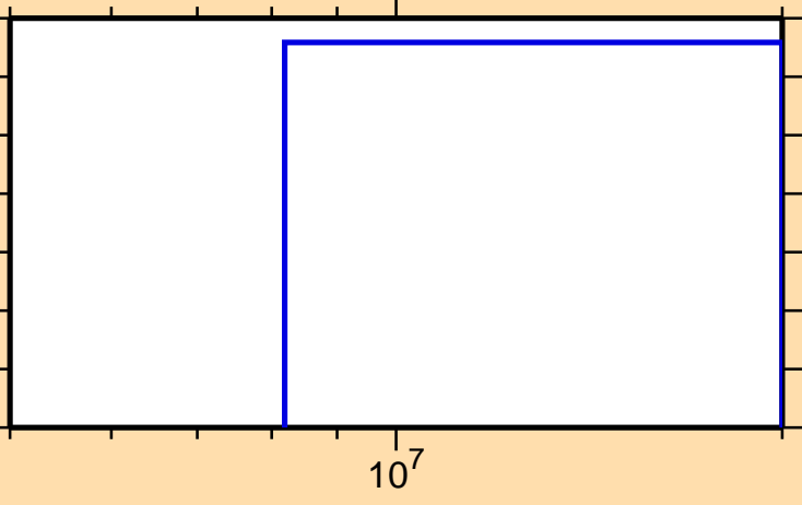
\sigma vs. E for ^{144}\text{Pm}(n,2np)
