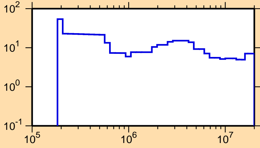
\Delta\sigma/\sigma vs. E for ^{145}\text{Pm}(n,el.)
