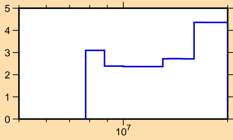
\Delta\sigma/\sigma vs. E for ^{145}\text{Pm}(n,\text{tot.})
