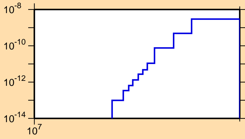
\sigma vs. E for ^{145}\text{Pm} (mt 45)
