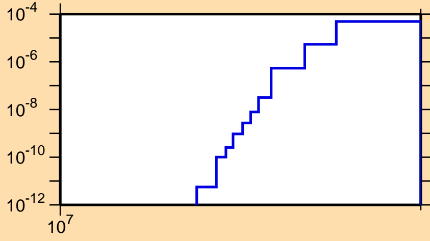
\sigma vs. E for ^{145}\text{Pm}(n,nd)
