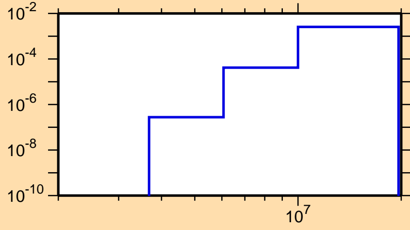
\sigma vs. E for ^{145}\text{Pm}(n,n\alpha)
