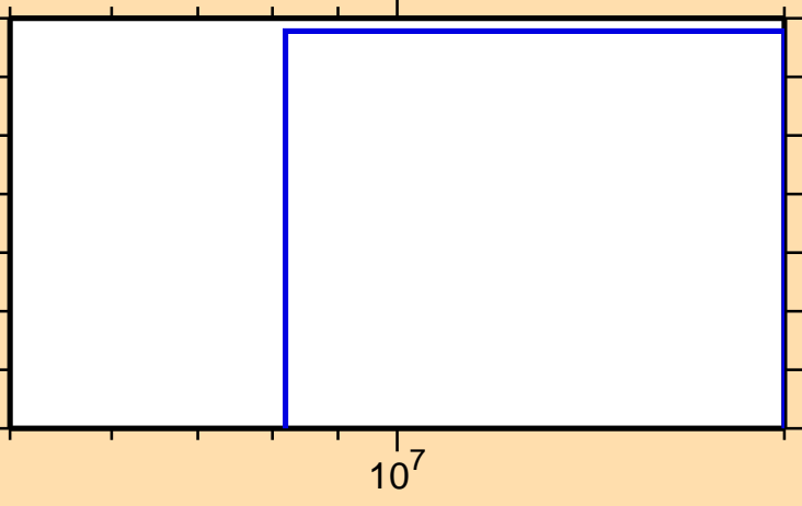
\sigma vs. E for ^{145}\text{Pm}(n,\text{nd})
