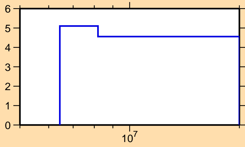
\Delta\sigma/\sigma vs. E for ^{145}\text{Pm}(n,\text{el.})
