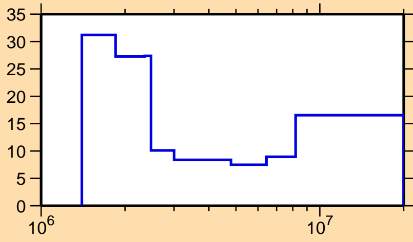
\Delta\sigma/\sigma vs. E for ^{145}\text{Pm}(n,n\text{cont.})
