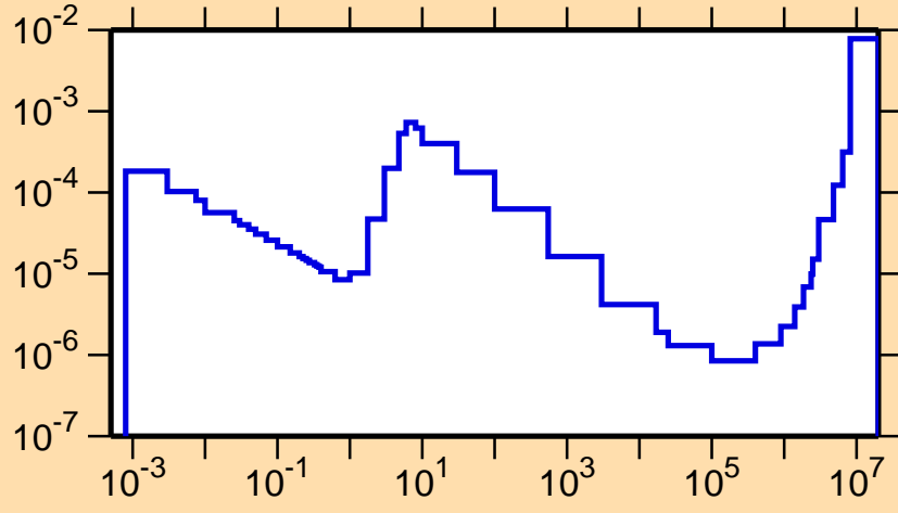
\sigma vs. E for ^{145}\text{Pm}(n,\alpha)
