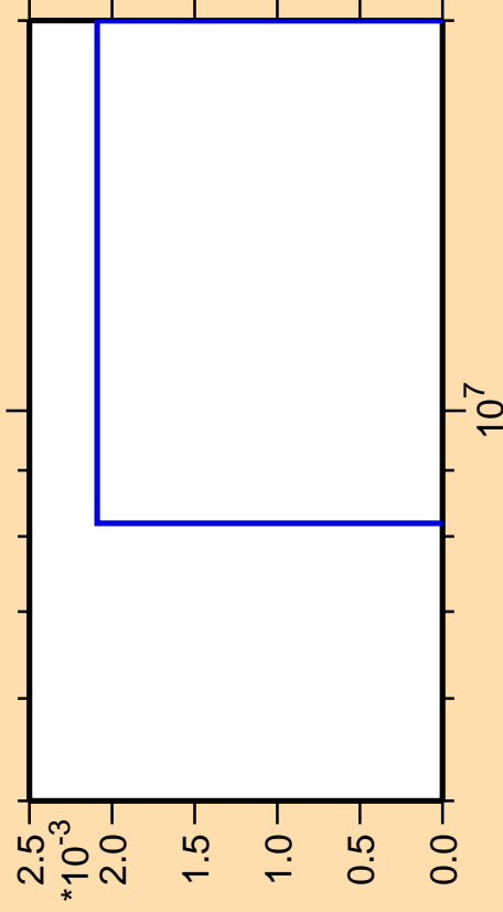
\Delta\sigma/\sigma vs. E for ^{145}\text{Pm} (mt 11)
