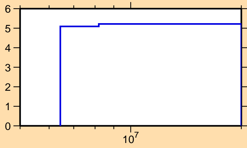
\Delta\sigma/\sigma vs. E for ^{145}\text{Pm}(n,\text{nonel.})
