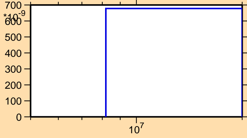
\sigma vs. E for ^{145}\text{Pm}(n,\text{nd})
