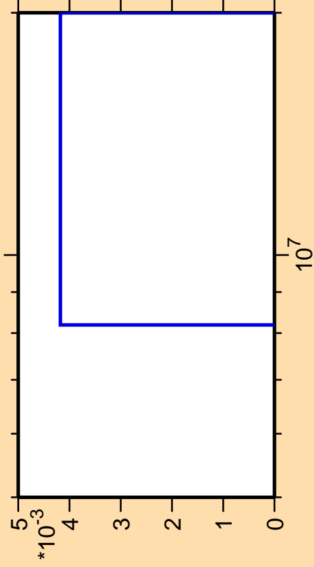
\Delta\sigma/\sigma vs. E for ^{145}\text{Pm}(n,pd)
