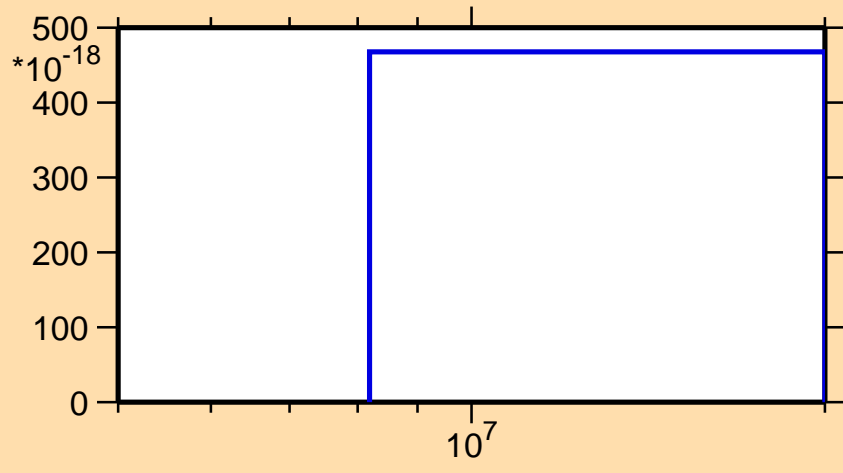
\sigma vs. E for ^{145}\text{Pm} (mt 34)
