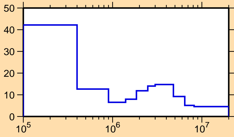
\Delta\sigma/\sigma vs. E for ^{145}\text{Pm}(n,el.)
