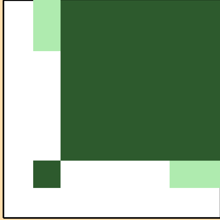
\sigma vs. E for ^{146}\text{Pm}(n,2np)
