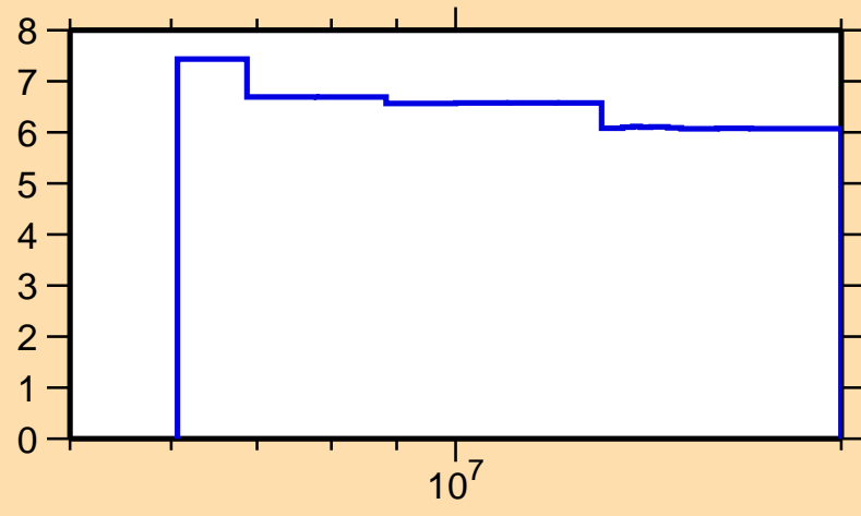
\Delta\sigma/\sigma vs. E for ^{146}\text{Pm}(n,\text{nonel.})
