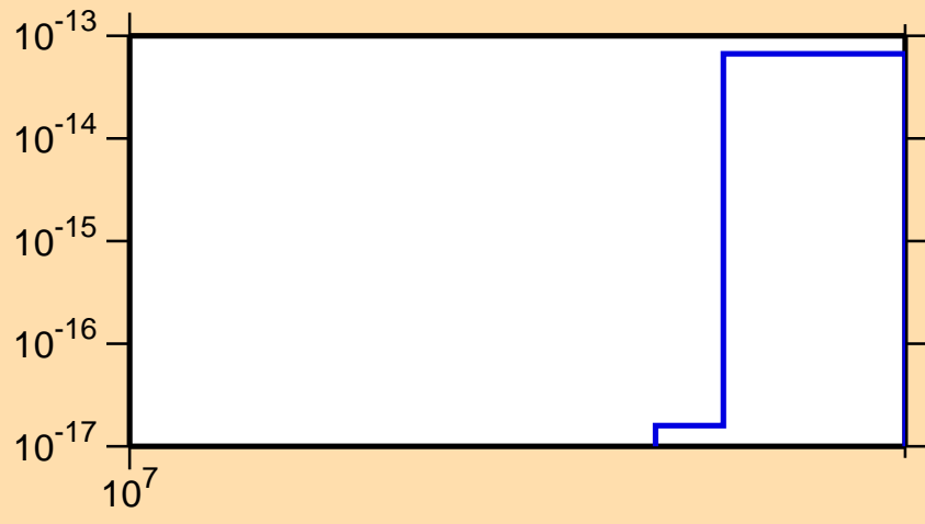
\sigma vs. E for ^{146}\text{Pm} (mt 11)
