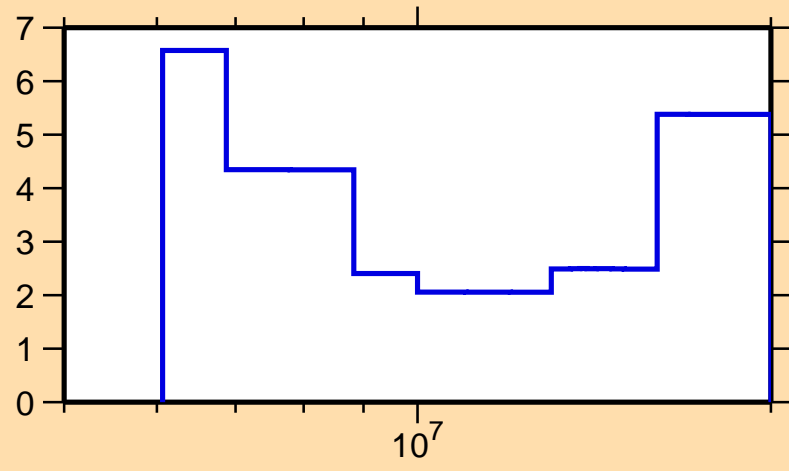
\Delta\sigma/\sigma vs. E for ^{146}\text{Pm}(n,\text{tot.})
