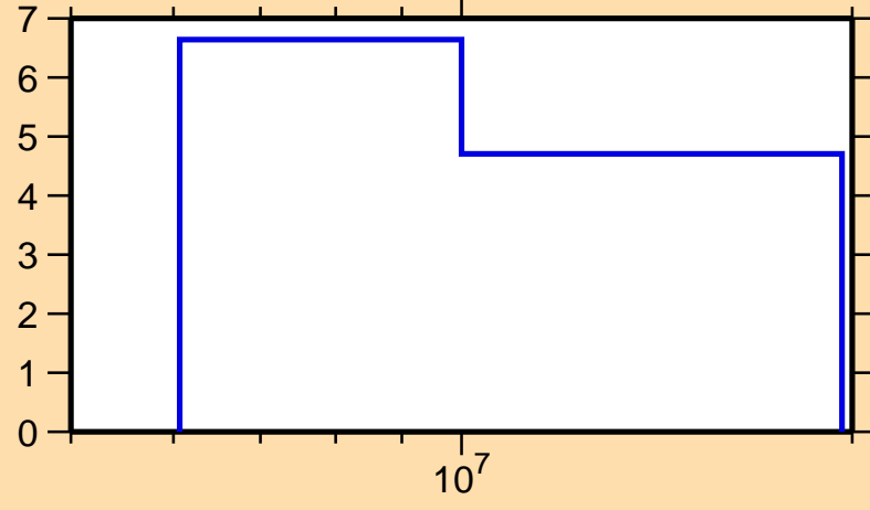
\Delta\sigma/\sigma vs. E for ^{146}\text{Pm}(n,\text{el.})
