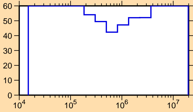
\Delta\sigma/\sigma vs. E for ^{146}\text{Pm}(n,n_1)
