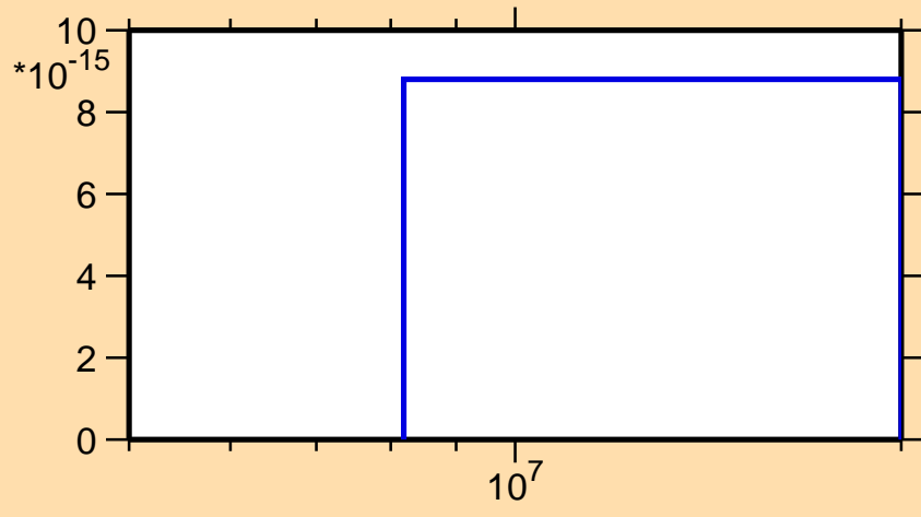
\sigma vs. E for ^{146}\text{Pm} (mt 34)
