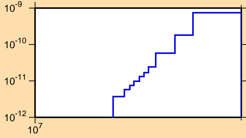
\sigma vs. E for ^{147}\text{Pm}(n,p\alpha)
