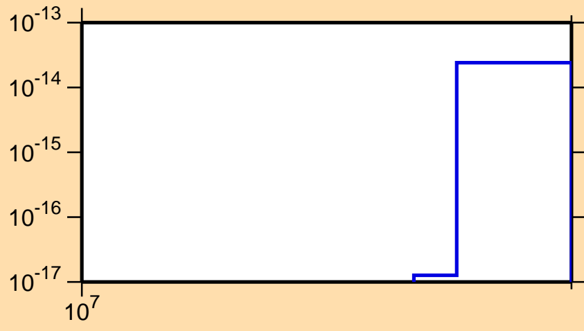
\sigma vs. E for ^{147}\text{Pm} (mt 11)
