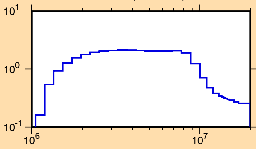
\sigma vs. E for ^{147}\text{Pm}(n,n\text{cont.})
