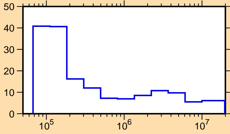
\Delta\sigma/\sigma vs. E for ^{147}\text{Pm}(n,el.)
