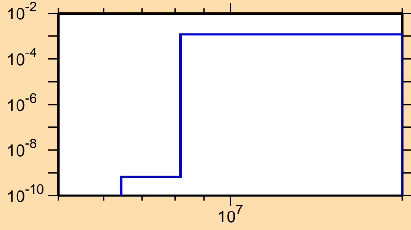
\sigma vs. E for ^{147}\text{Pm}(n,np)
