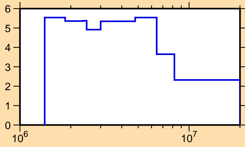
\Delta\sigma/\sigma vs. E for ^{147}\text{Pm}(n,\text{tot.})
