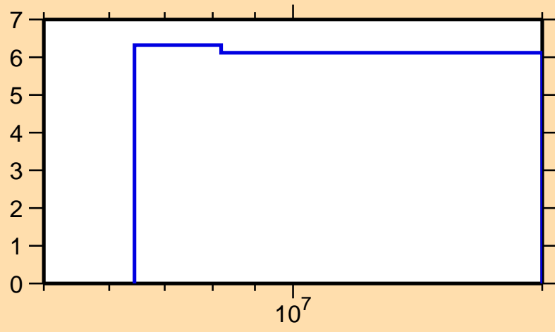
\Delta\sigma/\sigma vs. E for ^{147}\text{Pm}(n,\text{el.})
