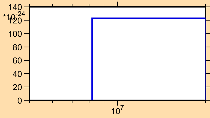
\sigma vs. E for ^{147}\text{Pm} (mt 42)
