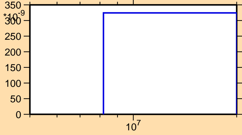
\sigma vs. E for ^{147}\text{Pm}(n,nd)
