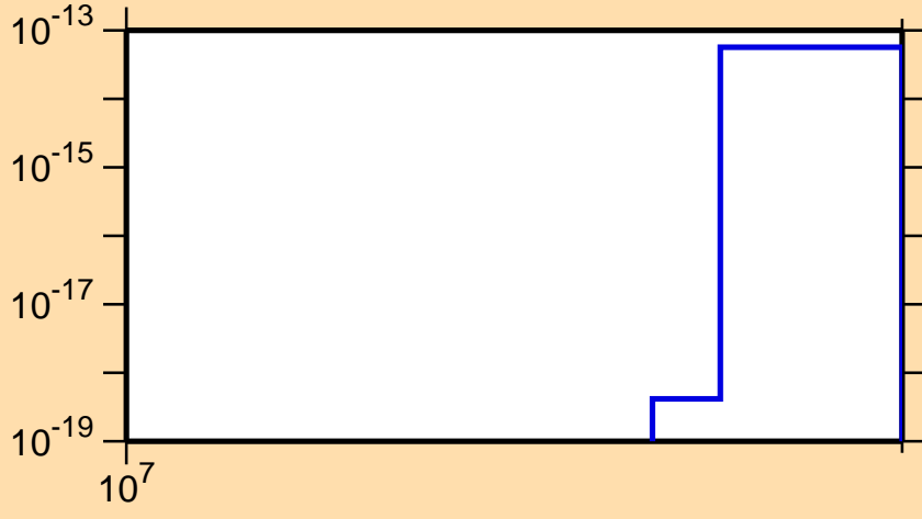
\sigma vs. E for ^{148}\text{Pm} (mt 34)
