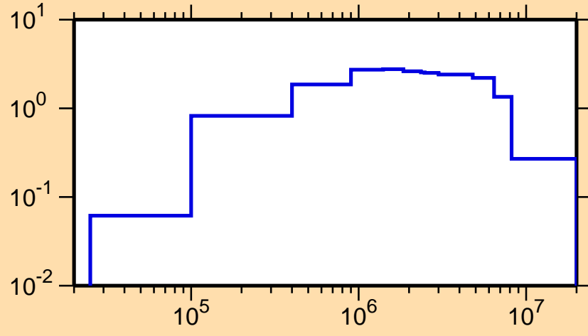
\sigma vs. E for ^{148}\text{Pm}(n,\text{inel.})
