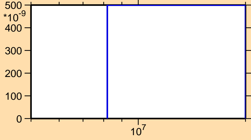
\sigma vs. E for ^{148}\text{Pm}(n,nt)
