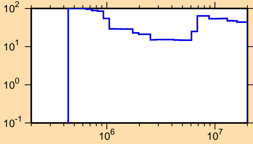
\Delta\sigma/\sigma vs. E for ^{148}\text{Pm}(n,n\text{cont.})
