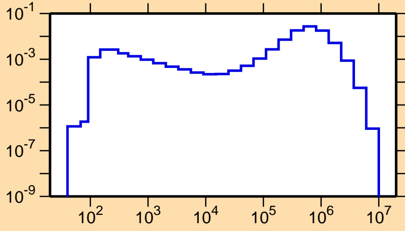
\sigma vs. E for ^{148}\text{Pm}(n,n_1)
