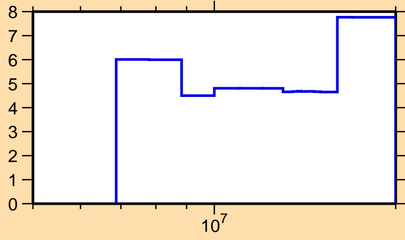
\Delta\sigma/\sigma vs. E for ^{149}\text{Pm}(n,\text{tot.})
