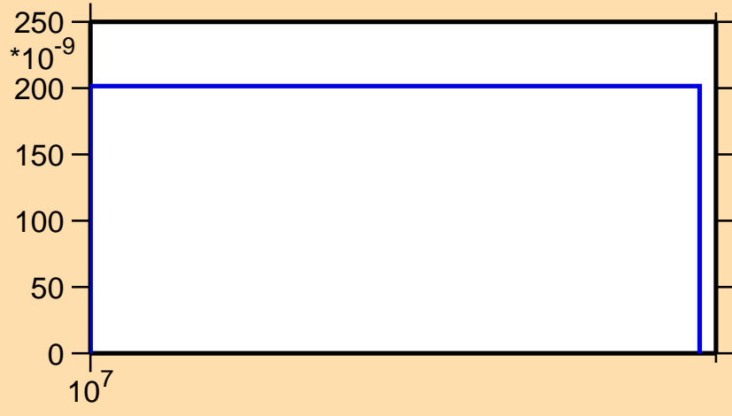
\sigma vs. E for ^{149}\text{Pm}(n,nd)
