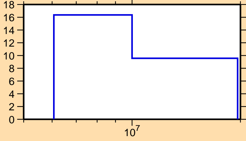
\Delta\sigma/\sigma vs. E for ^{149}\text{Pm}(n,el.)
