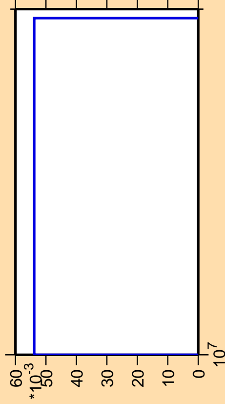
\Delta\sigma/\sigma vs. E for ^{149}\text{Pm}(\text{mt117})
