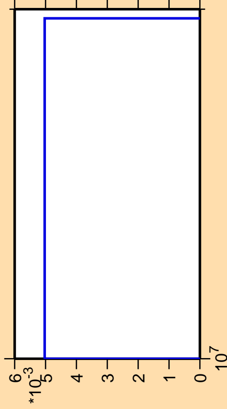
\Delta\sigma/\sigma vs. E for ^{149}\text{Pm} (mt 11)
