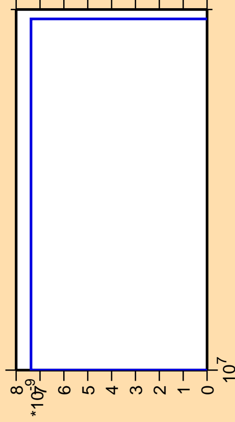
\Delta\sigma/\sigma vs. E for ^{149}\text{Pm} (mt 42)
