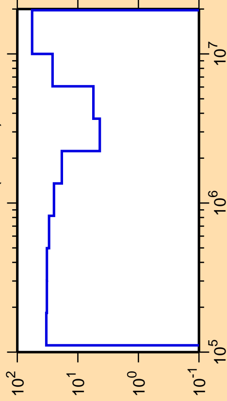
\Delta\sigma/\sigma vs. E for ^{149}\text{Pm}(n,\text{inel.})
