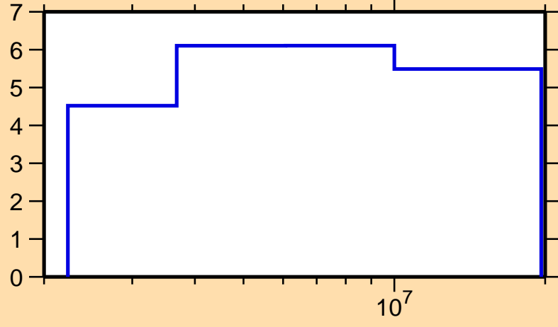
\Delta\sigma/\sigma vs. E for ^{149}\text{Pm}(n,\text{nonel.})
