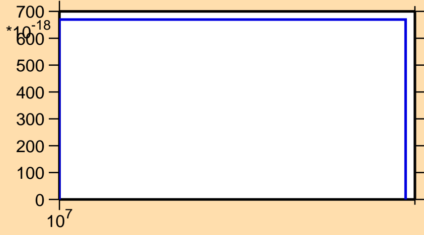
\sigma vs. E for ^{149}\text{Pm} (mt 11)
