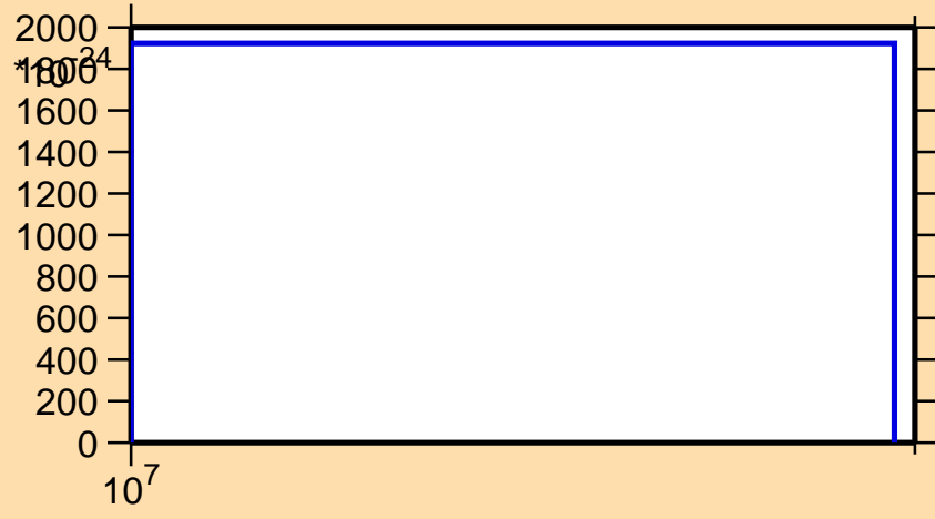
\sigma vs. E for ^{149}\text{Pm} (mt 42)
