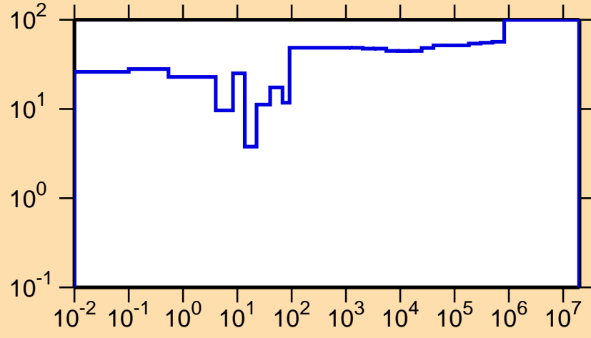
\Delta\sigma/\sigma vs. E for ^{149}\text{Pm}(n,\gamma)
