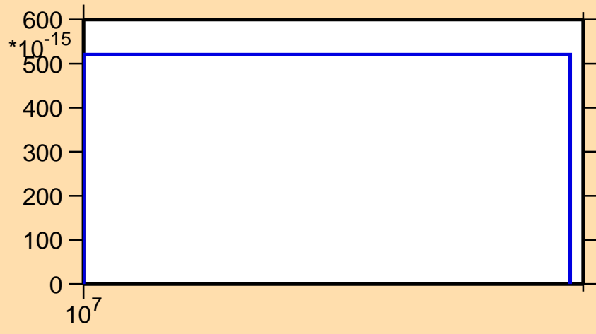
\sigma vs. E for ^{149}\text{Pm}(n,p\alpha)
