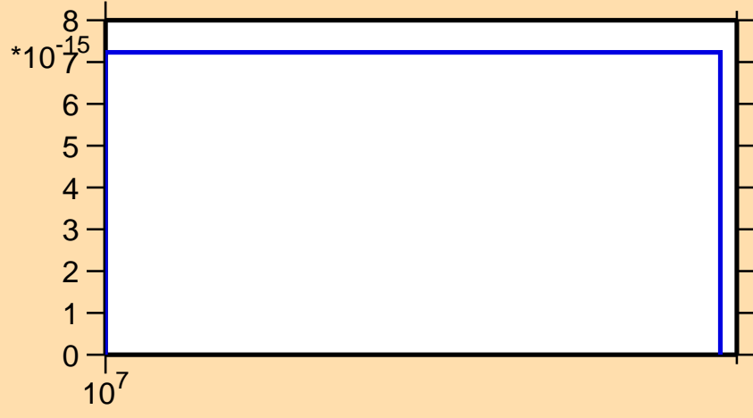
\sigma vs. E for ^{149}\text{Pm}(\text{mt117})
