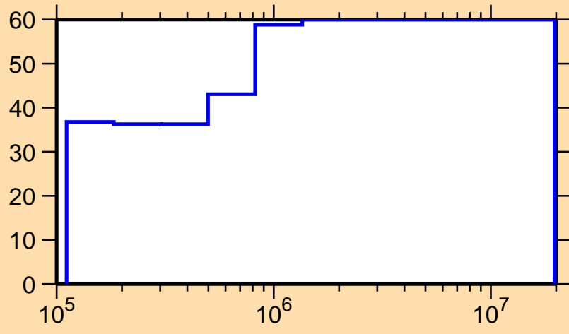
\Delta\sigma/\sigma vs. E for ^{149}\text{Pm}(n,n_1)
