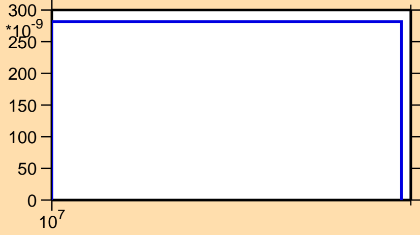
\sigma vs. E for ^{149}\text{Pm}(n,nt)
