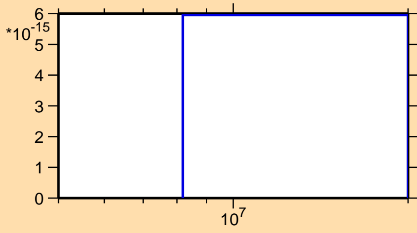
\sigma vs. E for ^{149}\text{Pm}(\text{mt117})
