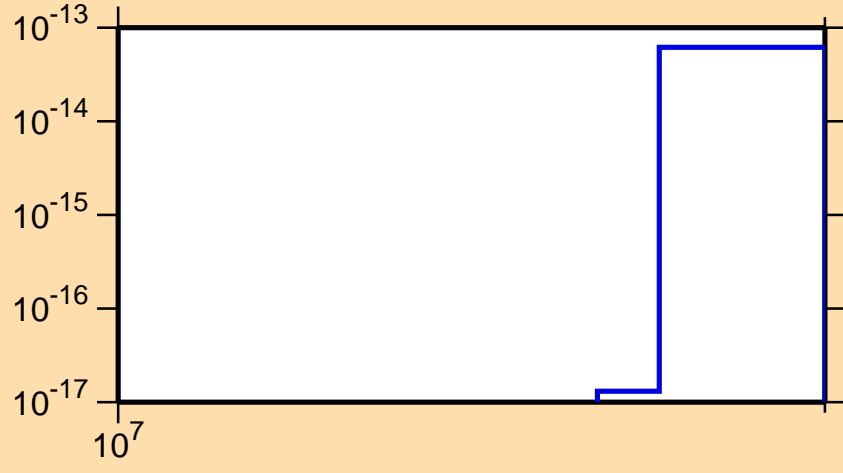
\sigma vs. E for ^{150}\text{Pm} (mt 11)
