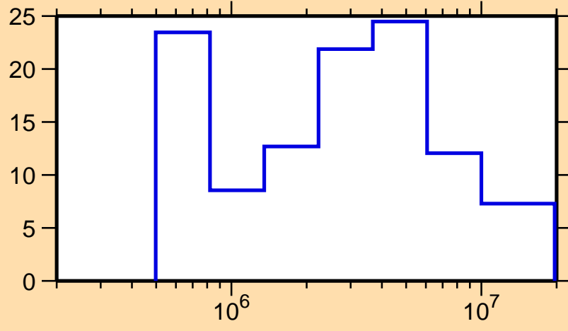
\Delta\sigma/\sigma vs. E for ^{150}\text{Pm}(n,el.)
