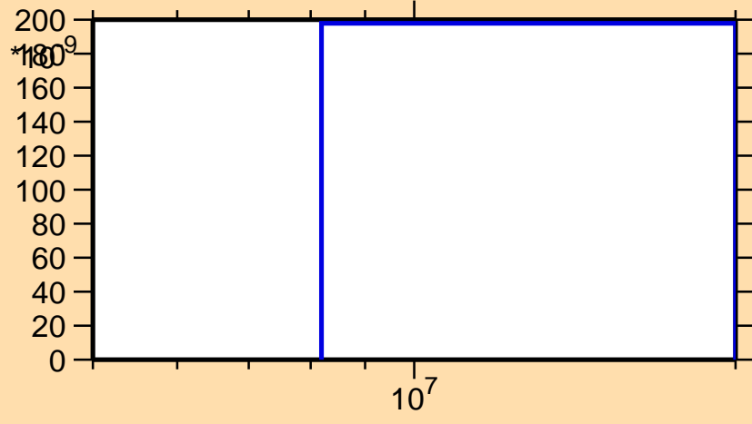
\sigma vs. E for ^{150}\text{Pm}(n,2np)
