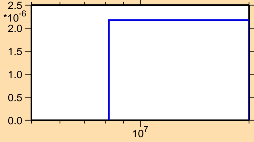
\sigma vs. E for ^{150}\text{Pm}(n,nd)
