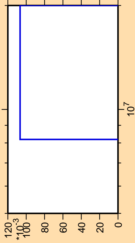
\Delta\sigma/\sigma vs. E for ^{150}\text{Pm}(n,3n\alpha)
