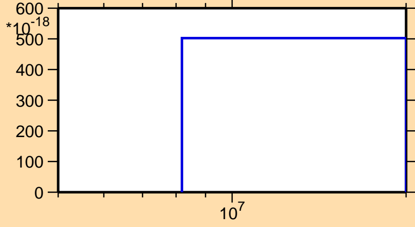
\sigma vs. E for ^{150}\text{Pm} (mt 11)
