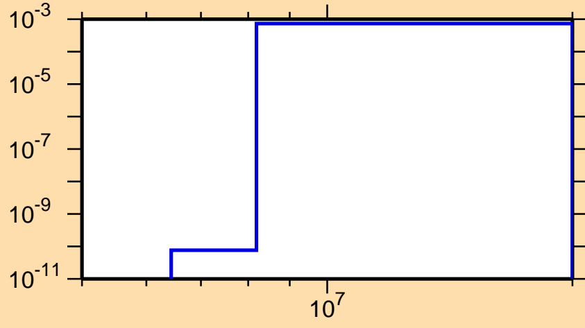
\sigma vs. E for ^{150}\text{Pm}(n,d)
