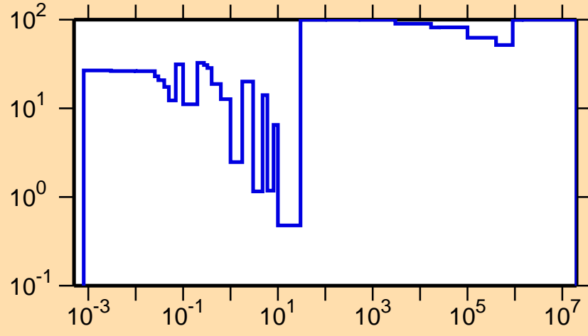
\Delta\sigma/\sigma vs. E for ^{150}\text{Pm}(n,\gamma)
