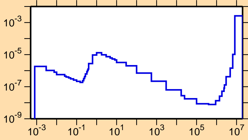
\sigma vs. E for ^{150}\text{Pm}(n,\alpha)
