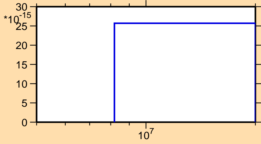
\sigma vs. E for ^{150}\text{Pm}(n,3n\alpha)
