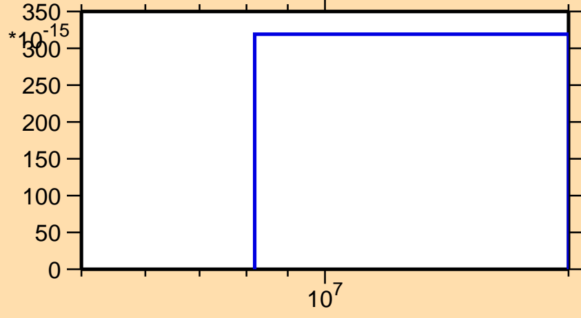
\sigma vs. E for ^{150}\text{Pm}(n,p\alpha)
