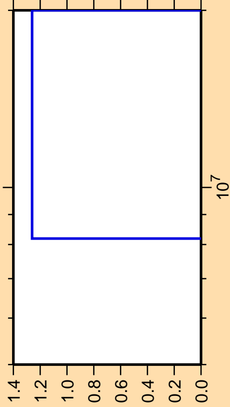
\Delta\sigma/\sigma vs. E for ^{150}\text{Pm}(n,p\alpha)
