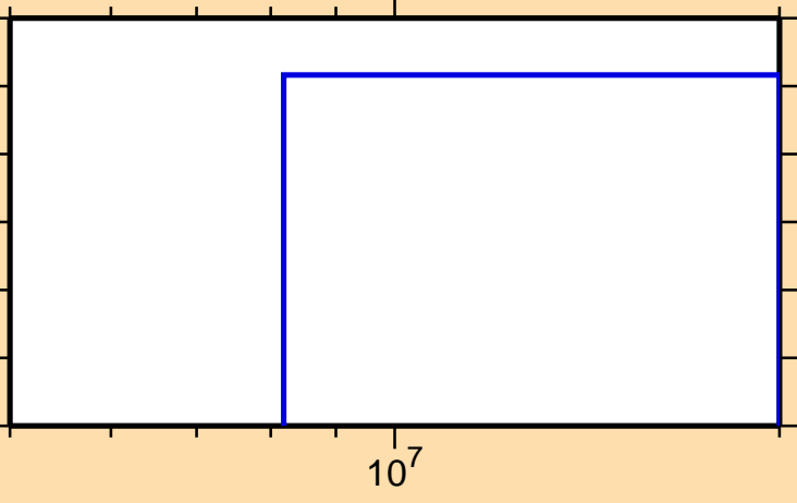
\sigma vs. E for ^{150}\text{Pm}(n,2n\alpha)
