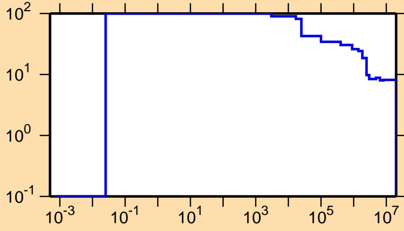
\Delta\sigma/\sigma vs. E for ^{150}\text{Pm}(n,\text{nonel.})
