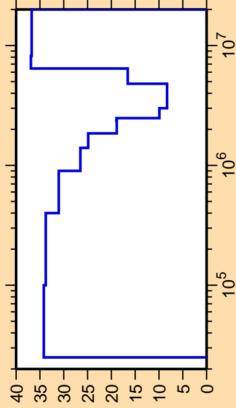
\Delta\sigma/\sigma vs. E for ^{150}\text{Pm}(n,\text{inel.})
