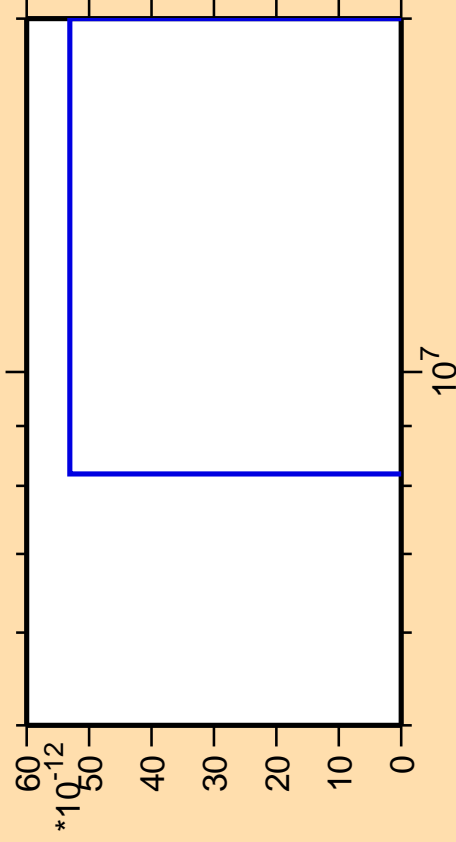
\Delta\sigma/\sigma vs. E for ^{150}\text{Pm} (mt 42)
