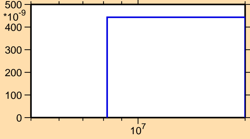
\sigma vs. E for ^{150}\text{Pm}(n,nt)
