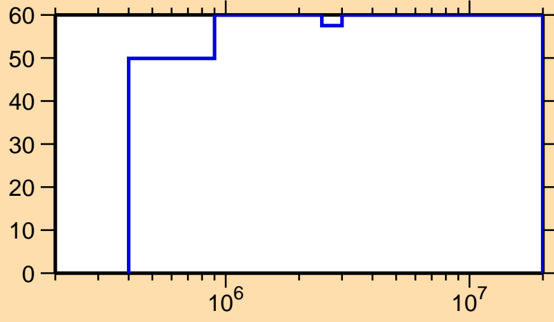
\Delta\sigma/\sigma vs. E for ^{150}\text{Pm}(n,n_1)
