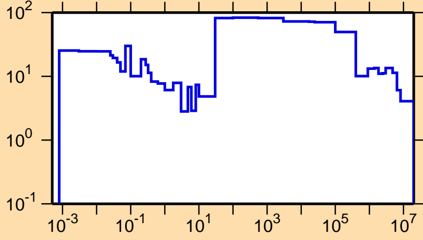
\Delta\sigma/\sigma vs. E for ^{150}\text{Pm}(n,\text{tot.})
