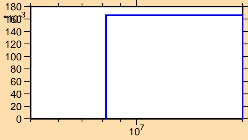
\sigma vs. E for ^{150}\text{Pm}(n,3n)
