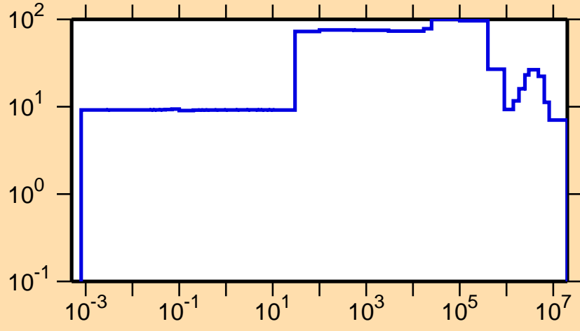
\Delta\sigma/\sigma vs. E for ^{150}\text{Pm}(n,\text{el.})
