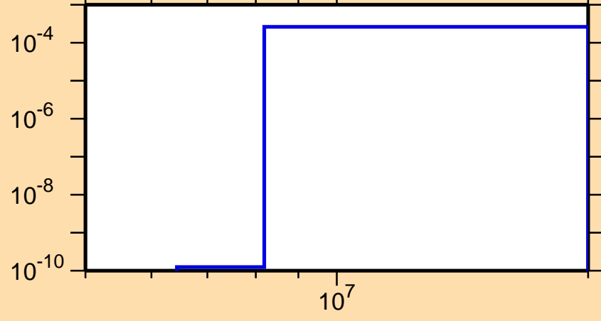
\sigma vs. E for ^{150}\text{Pm}(n,t)
