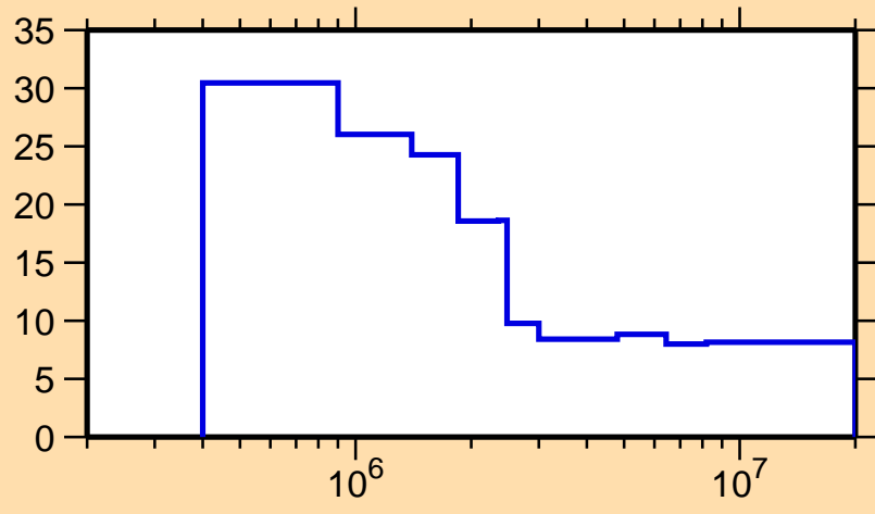
\Delta\sigma/\sigma vs. E for ^{150}\text{Pm}(n,\text{nonel.})
