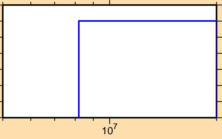
\sigma vs. E for ^{150}\text{Pm} (mt 42)
