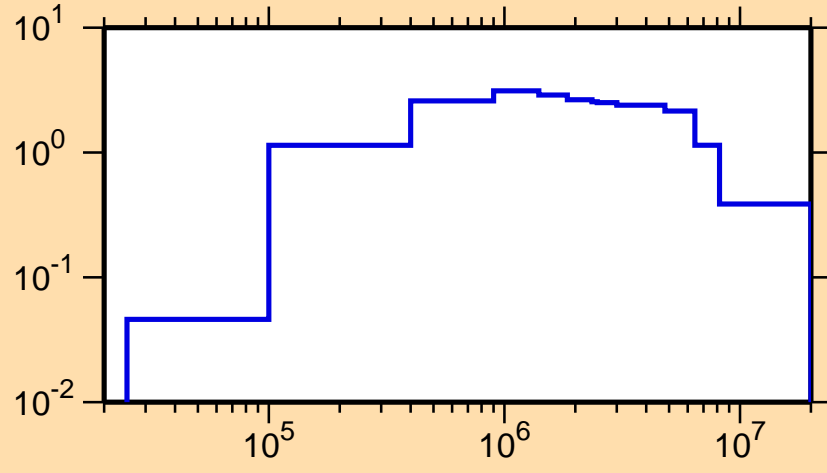
\sigma vs. E for ^{150}\text{Pm}(n,\text{inel.})
