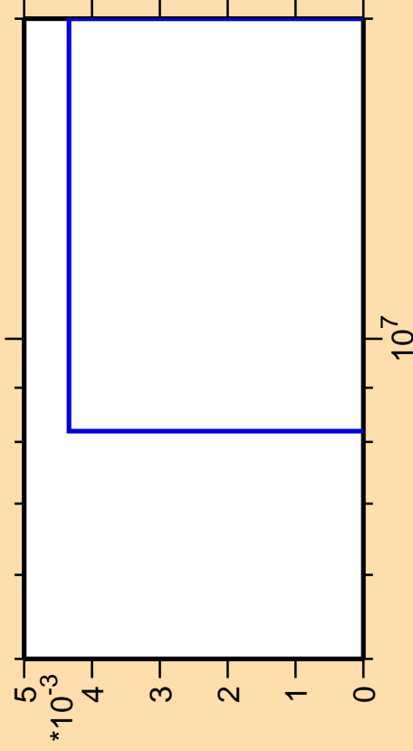
\Delta\sigma/\sigma vs. E for ^{150}\text{Pm} (mt 11)
