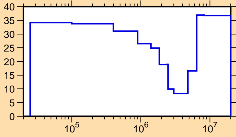
\Delta\sigma/\sigma vs. E for ^{150}\text{Pm}(n,\text{inel.})
