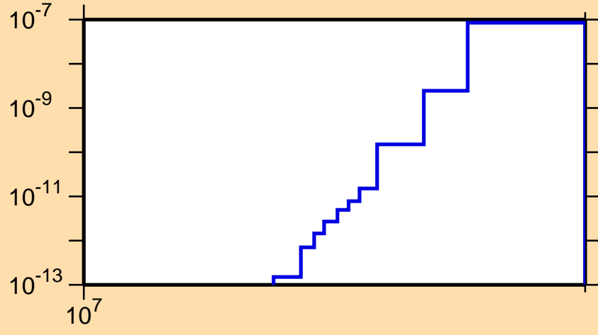
\sigma vs. E for ^{151}\text{Pm}(n,2n\alpha)
