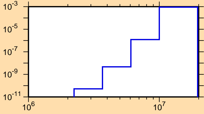
\sigma vs. E for ^{151}\text{Pm}(n,\alpha)
