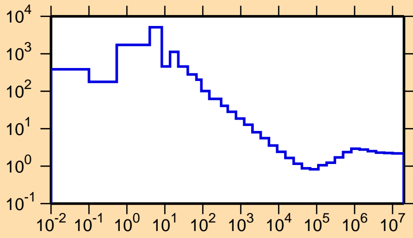
\sigma vs. E for ^{151}\text{Pm}(n,\text{nonel.})
