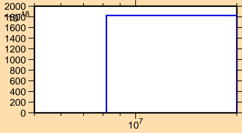
\sigma vs. E for ^{151}\text{Pm}(n,3n\alpha)
