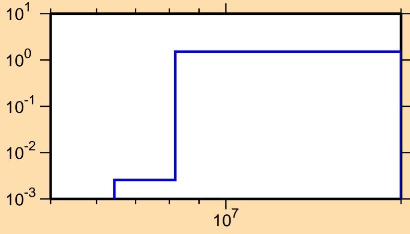
\sigma vs. E for ^{151}\text{Pm}(n,2n)
