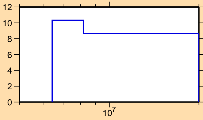
\Delta\sigma/\sigma vs. E for ^{151}\text{Pm}(n,\text{nonel.})
