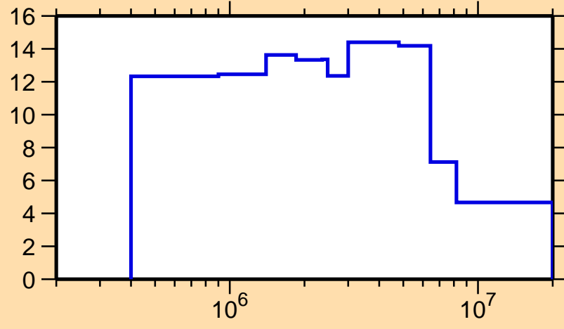
\Delta\sigma/\sigma vs. E for ^{151}\text{Pm}(n,\text{tot.})
