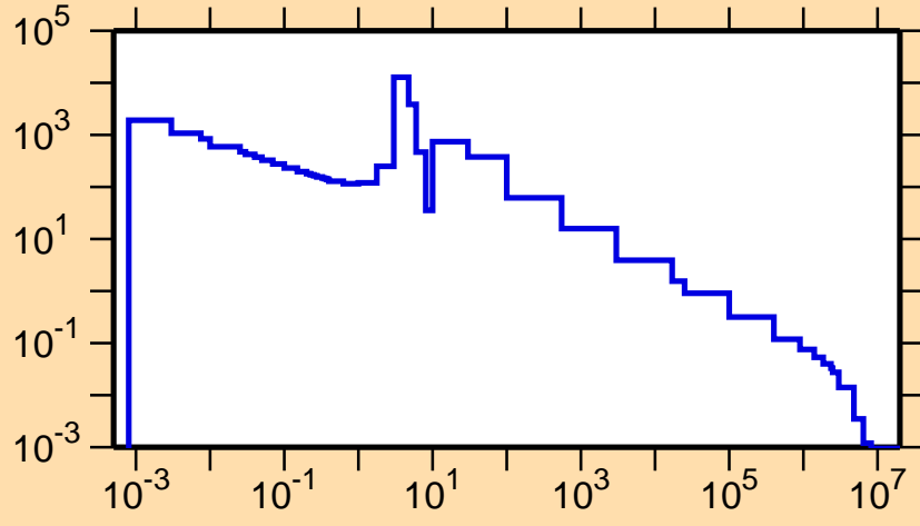
\sigma vs. E for ^{151}\text{Pm}(n,\gamma)
