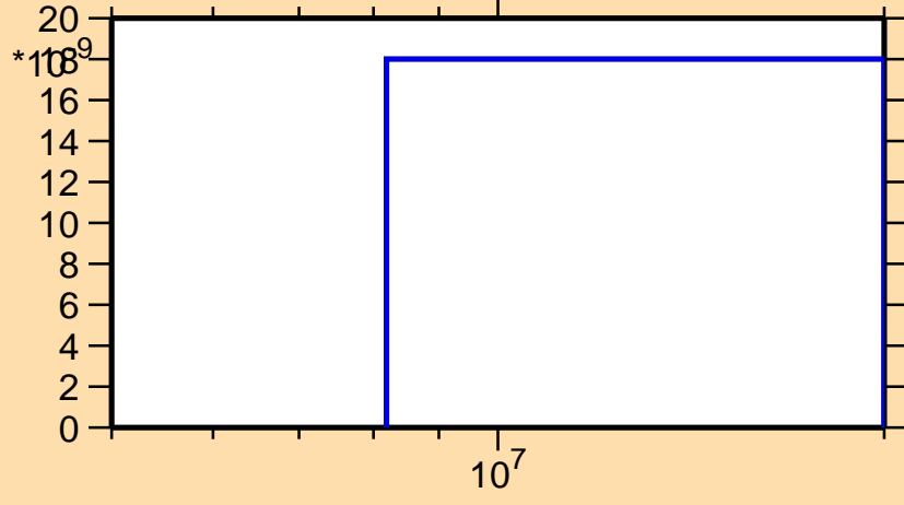
\sigma vs. E for ^{151}\text{Pm}(n,\text{nd})
