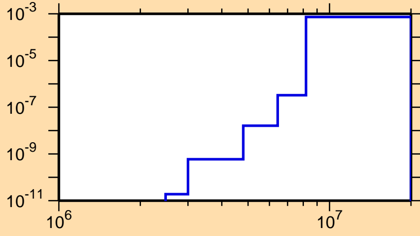
\sigma vs. E for ^{151}\text{Pm}(n,\alpha)
