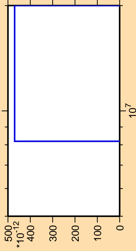
\Delta\sigma/\sigma vs. E for ^{151}\text{Pm} (mt 42)
