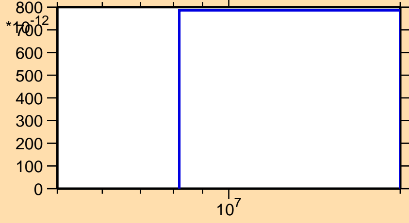
\sigma vs. E for ^{151}\text{Pm}(n,2np)
