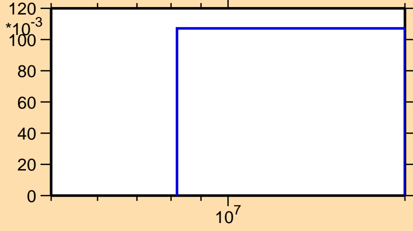
\sigma vs. E for ^{151}\text{Pm}(n,3n)
