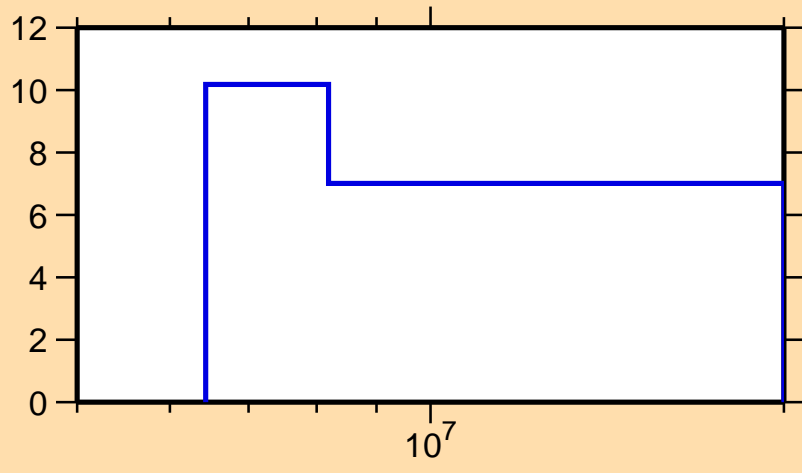
\Delta\sigma/\sigma vs. E for ^{151}\text{Pm}(n,\text{el.})
