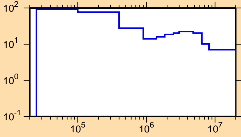
\Delta\sigma/\sigma vs. E for ^{151}\text{Pm}(n,\text{el.})
