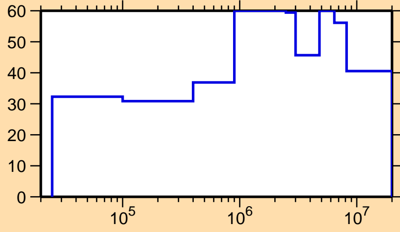
\Delta\sigma/\sigma vs. E for ^{151}\text{Pm}(n,n_1)
