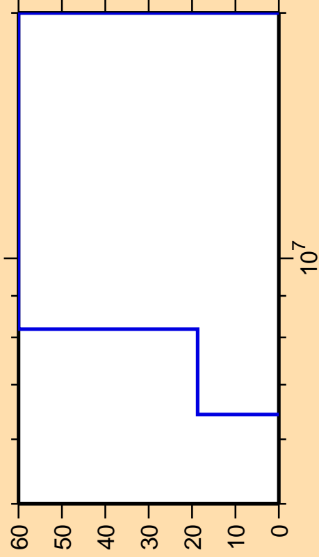
\Delta\sigma/\sigma vs. E for ^{151}\text{Pm}(n,n_{\text{cont}})
