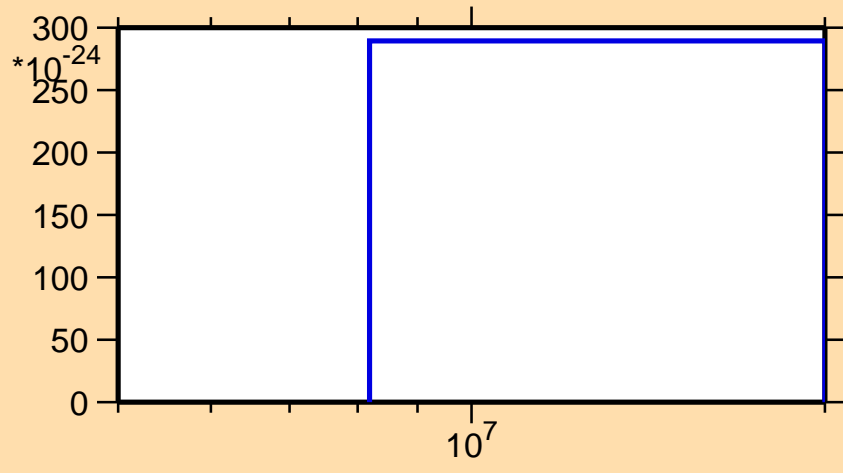
\sigma vs. E for ^{151}\text{Pm} (mt 42)
