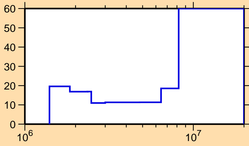
\Delta\sigma/\sigma vs. E for ^{151}\text{Pm}(n,\text{inel.})
