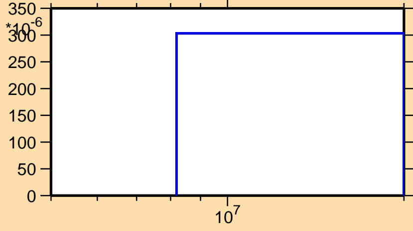
\sigma vs. E for ^{151}\text{Pm}(n,np)
