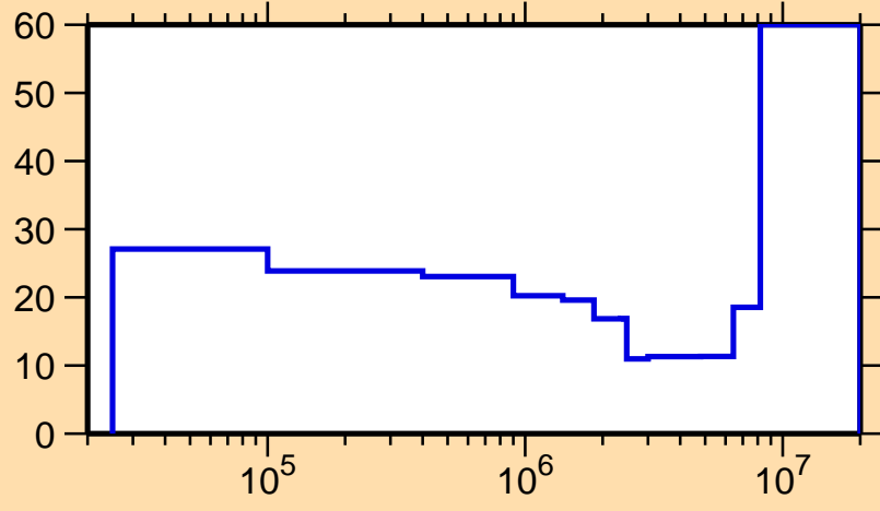
\Delta\sigma/\sigma vs. E for ^{151}\text{Pm}(n,\text{inel.})
