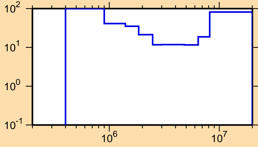
\Delta\sigma/\sigma vs. E for ^{151}\text{Pm}(n,n\text{cont.})
