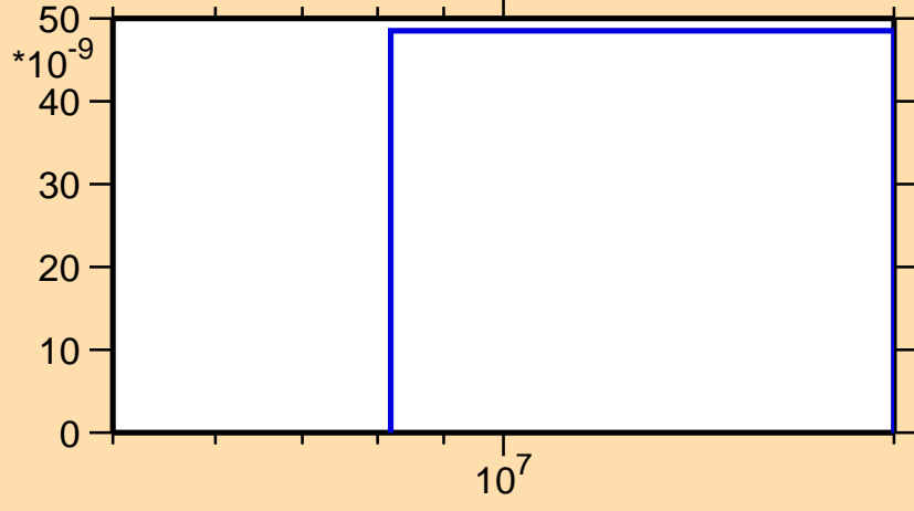
\sigma vs. E for ^{151}\text{Pm}(n,nt)
