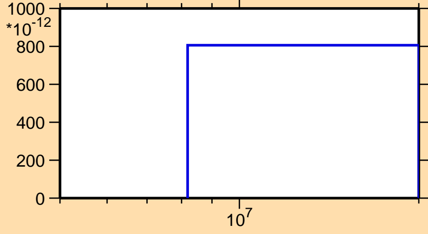
\sigma vs. E for ^{151}\text{Pm}(n,2n\alpha)
