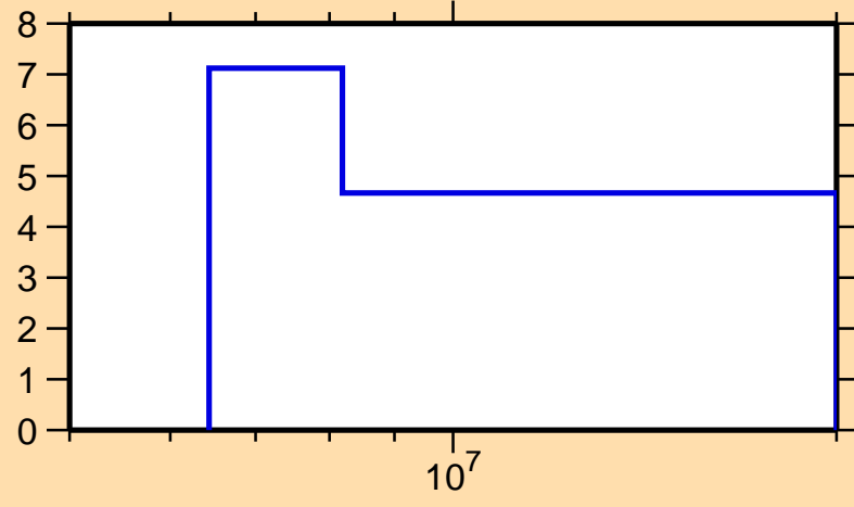
\Delta\sigma/\sigma vs. E for ^{151}\text{Pm}(n,\text{tot.})
