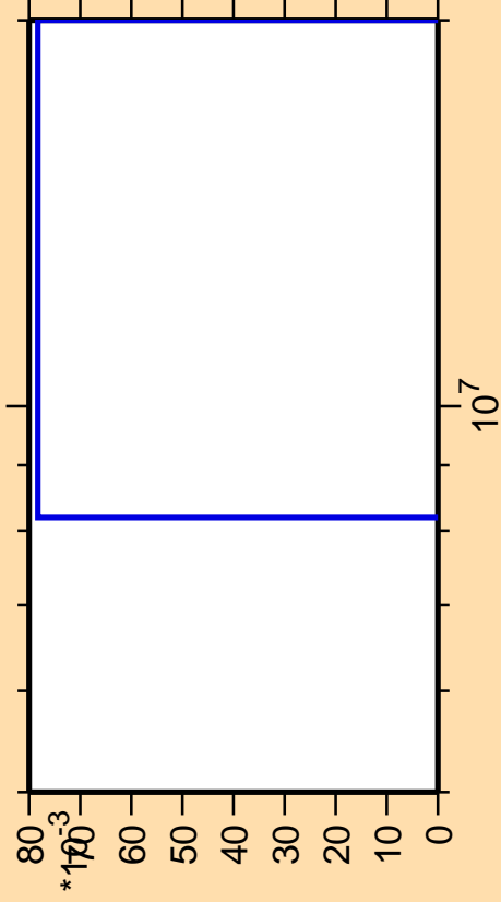
\Delta\sigma/\sigma vs. E for ^{151}\text{Pm}(n,\text{He}3)
