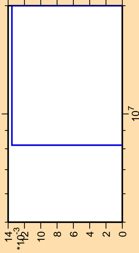
\Delta\sigma/\sigma vs. E for ^{151}\text{Pm}(n,3n\alpha)
