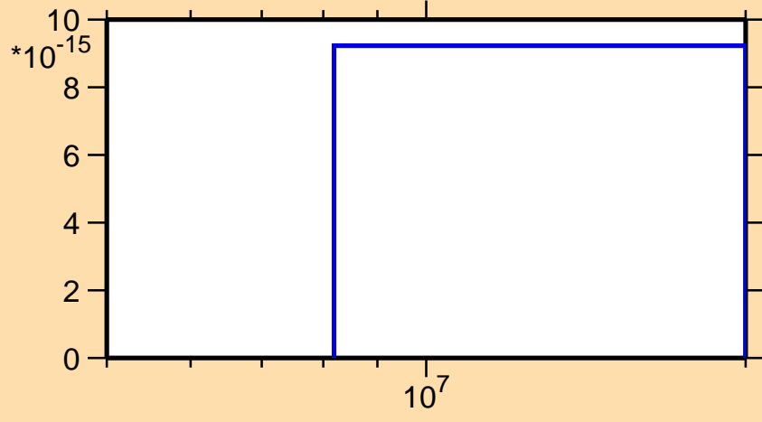
\sigma vs. E for ^{151}\text{Pm}(n,\text{He}3)
