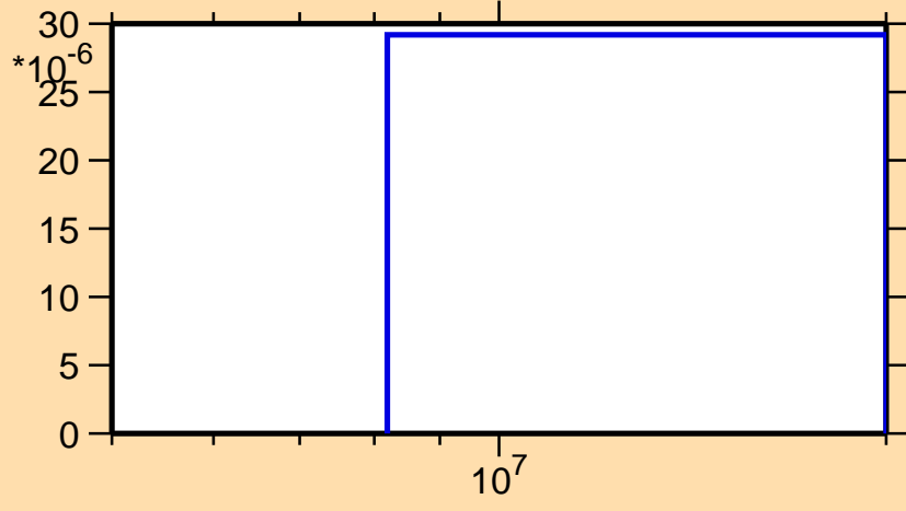
\sigma vs. E for ^{151}\text{Pm}(n,t)
