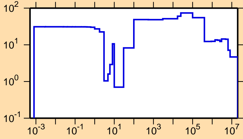
\Delta\sigma/\sigma vs. E for ^{151}\text{Pm}(n,\text{tot.})
