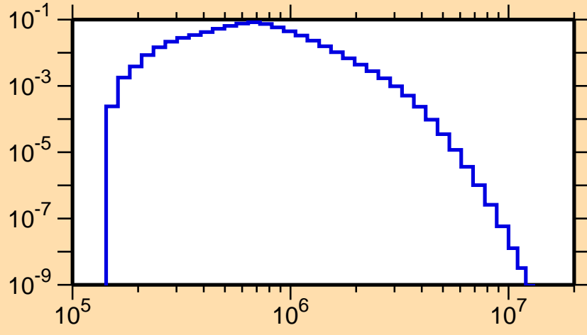
\sigma vs. E for ^{152}\text{Pm}(n,n_4)
