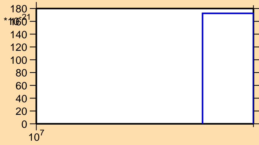
\sigma vs. E for ^{152}\text{Pm} (mt 11)
