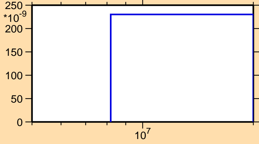
\sigma vs. E for ^{152}\text{Pm}(n,\text{nd})
