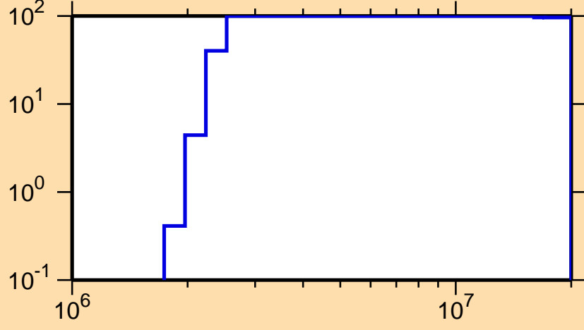
\Delta\sigma/\sigma vs. E for ^{152}\text{Pm}(n,p)
