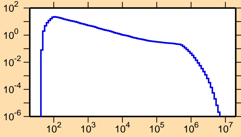
\sigma vs. E for ^{152}\text{Pm}(n,n_3)
