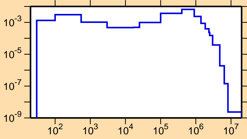
\sigma vs. E for ^{152}\text{Pm}(n,n_2)
