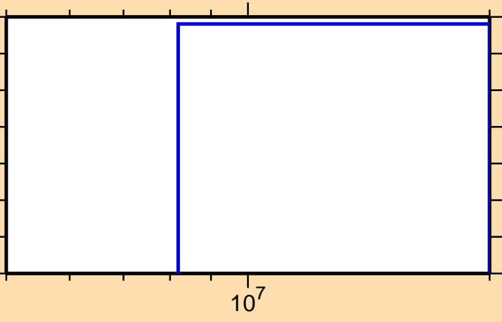
\sigma vs. E for ^{152}\text{Pm}(n,2n\alpha)
