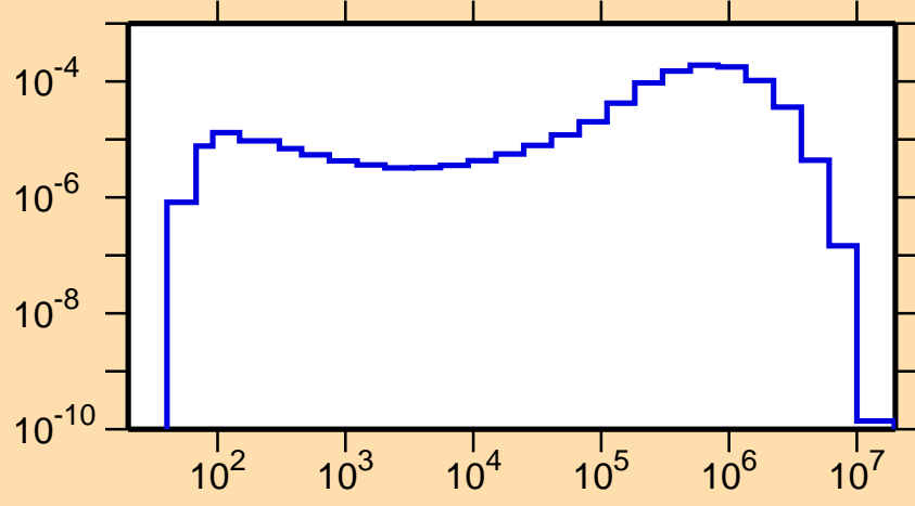
\sigma vs. E for ^{152}\text{Pm}(n,n_4)
