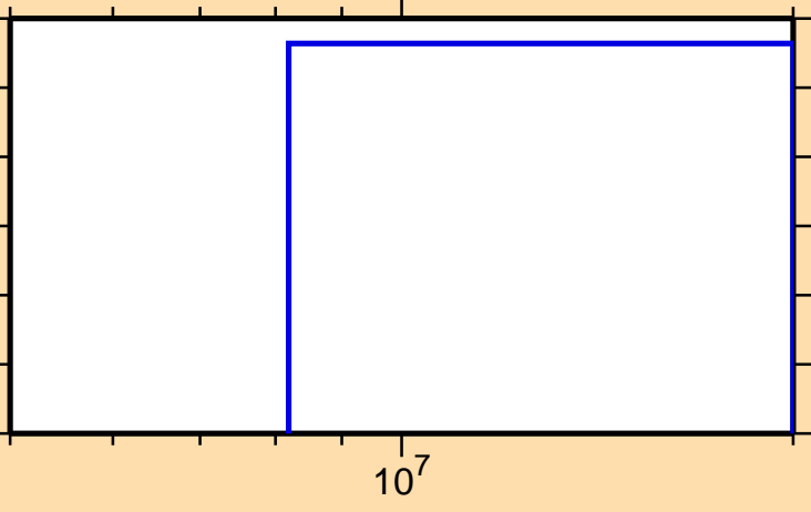
\sigma vs. E for ^{152}\text{Pm}(n,2n\alpha)
