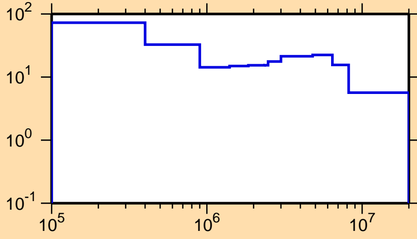
\Delta\sigma/\sigma vs. E for ^{152}\text{Pm}(n, el.)
