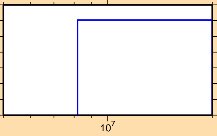
\sigma vs. E for ^{152}\text{Pm}(n,3n)
