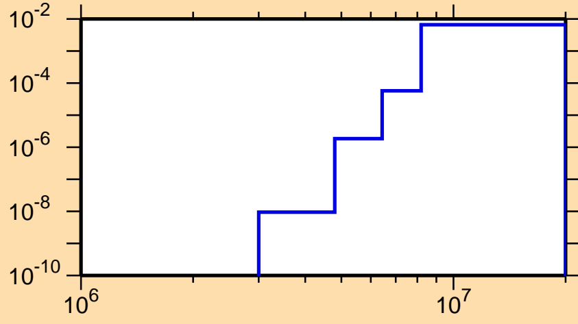
\sigma vs. E for ^{152}\text{Pm}(n,p)
