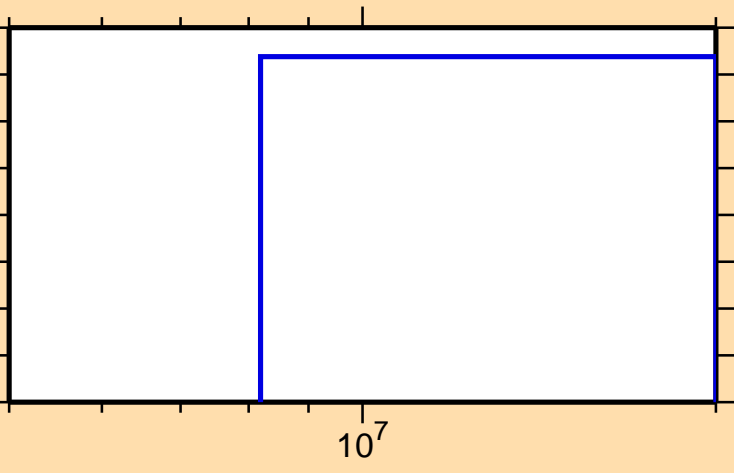
\sigma vs. E for ^{152}\text{Pm}(n,\text{He}3)
