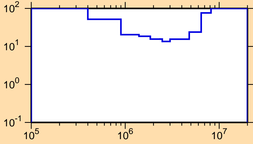
\Delta\sigma/\sigma vs. E for ^{152}\text{Pm}(n,n\text{cont.})
