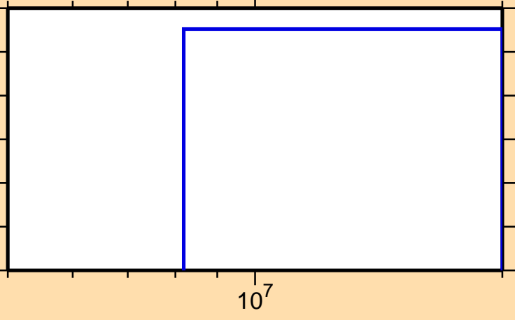
\sigma vs. E for ^{152}\text{Pm}(n,nt)
