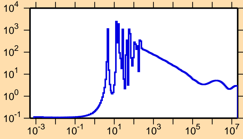
\sigma vs. E for ^{153}\text{Pm}(n,\text{el.})
