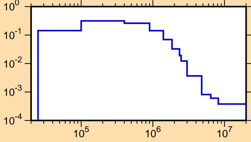
\sigma vs. E for ^{153}\text{Pm}(n,n_1)
