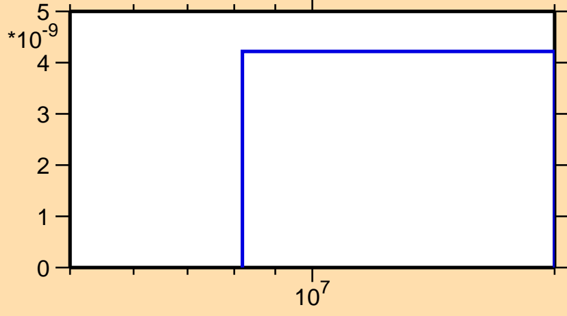
\sigma vs. E for ^{153}\text{Pm}(n,nd)
